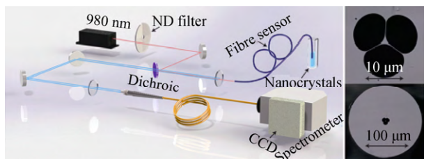
图 2 光纤颗粒负载法检测上转换发光实验系统示意图 [9] Fig. 2 Schematic experimental configuration for capturing UC luminescence of nanoparticles using a suspended-core microstructured optical-fiber dip sensor [9]
