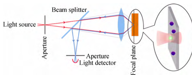
图 1 共聚焦显微荧光扫描系统原理示意图 Fig. 1 Schematic diagram of confocal microscopic fluorescent scanning system from upconversion nanoparticles
