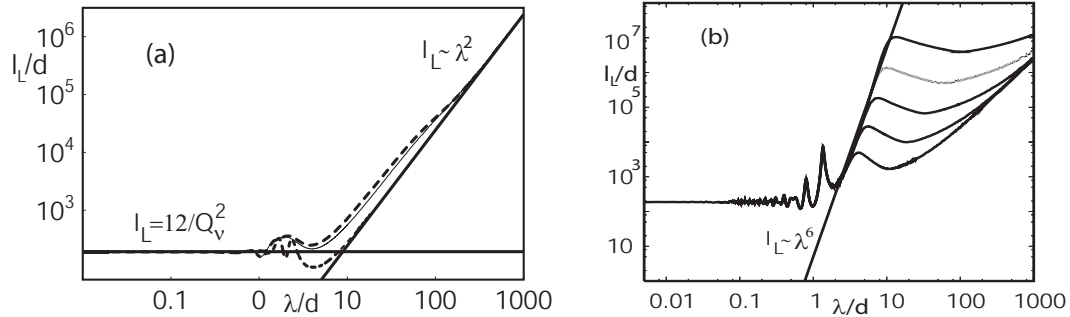
Fig. 1(a) Localisation length vs. wavelength for Q=0.25 , Q_d=0.2 for a M stack; thin solid line is the analytical prediction, top dashed line is the numerical simulation, lower dotted line is for the correspond H stack. Solid straight lines show short and long wavelength asymptotics. (b) l_L vs \lambda for stacks of length L = 10^s , s = 3, 4, 5, 6, 7 from bottom to top. The straight line is the \lambda^6 asymptotic.
