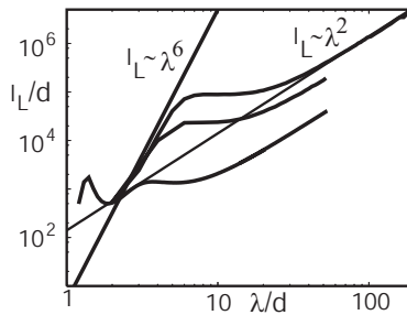
Fig. 2 l_L vs \lambda for stacks with Q_n=0.25 and Q_d=0.005, Q_d=0.01 and Q_d=0.05 from top to bottom.
