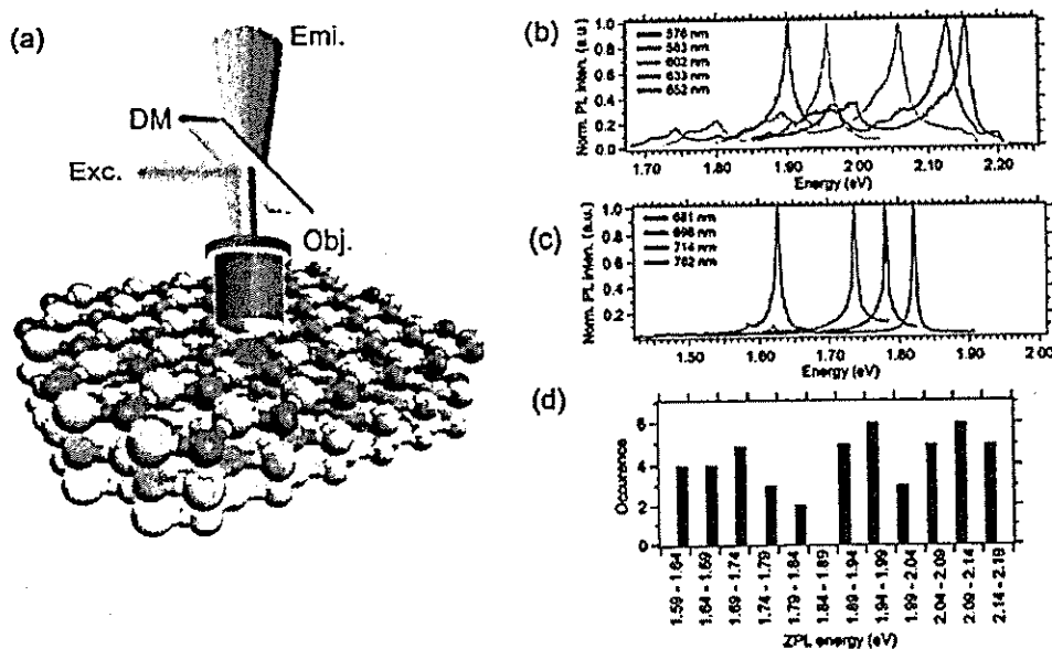
Figure 2 (a) Simplified schematic of the photoluminescence setup showing the excitation and emission of a defect center in a hBN lattice. The objective lens, dichroic mirror, excitation source and emission are denoted by Obj., DM, Exc., and Emi., respectively. (b) and (c) show nine examples of multicolor photoluminescence from point defects in hBN spanning a wide energy range (d) Histogram of ZPL energy for numerous emitters found in hBN. Figure modified from previous study. 5
