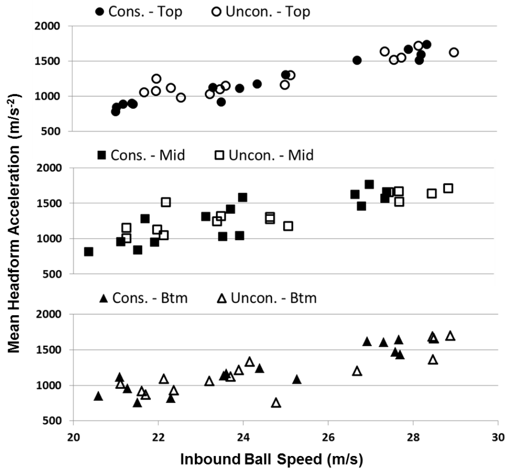
9 Figure 7. Comparison between mean resultant accelerations during the loading phase and 10 measured inbound ball speeds.
