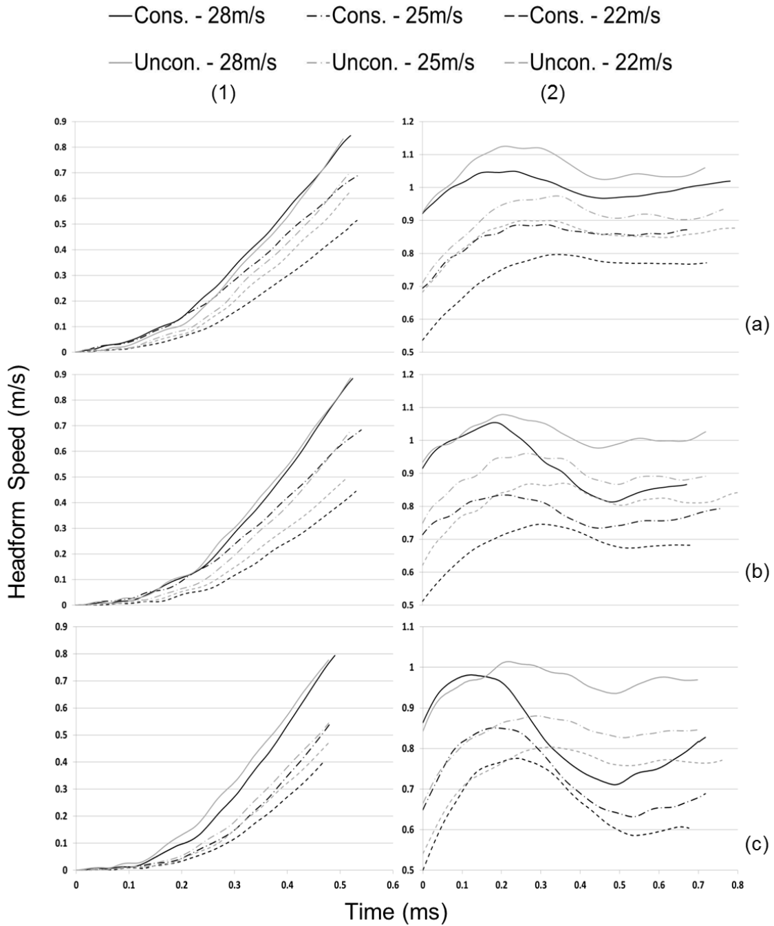
Figure 8. Comparison between mean speed traces at the Top (a), Middle (b) and Bottom (c) impact locations during the loading (1) and unloading (2) phases for the various mounting arrangement/impact speed combinations.
