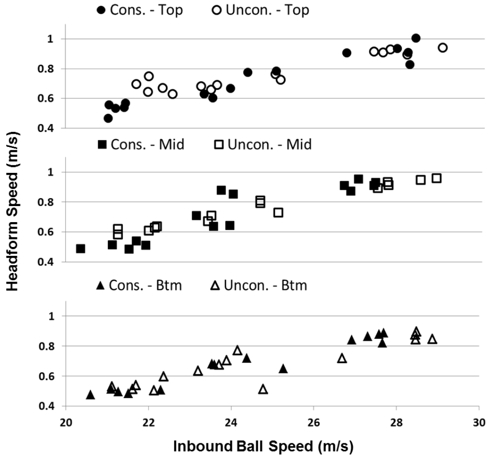
2 Figure 9. Comparison between headform speeds at peak ball deformation and measured 3 inbound ball speeds.
