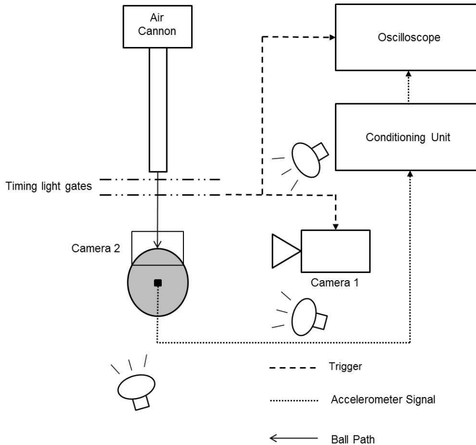
2 Figure 3. Schematic of the experimental arrangement.
