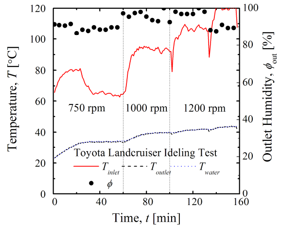
Figure 3. Transient test results for the Toyota LandCruiser engine at idling condition.
