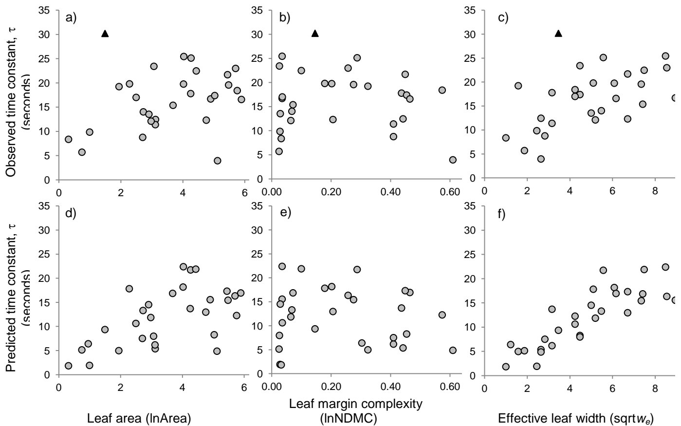
Figure 3. Comparison of the observed (a-c) vs predicted (d-f) time constant for leaf cooling ( \tau ) as a function of leaf area (a and d), margin complexity (NDMC, b and e) and effective leaf width ( w_e , c and f) for Proteaceae leaves in summer. Larger values for \tau denote slower leaf cooling speeds. The marked point in panels a-c (black triangle) is referred to in the Results. For analyses, all independent leaf traits were transformed to address non-normality, as indicated on the axes; however, for visual clarity, leaf area and NDMC are presented here as \ln(\text{Area}+1) and \ln(\text{NDMC}+1) , respectively.
