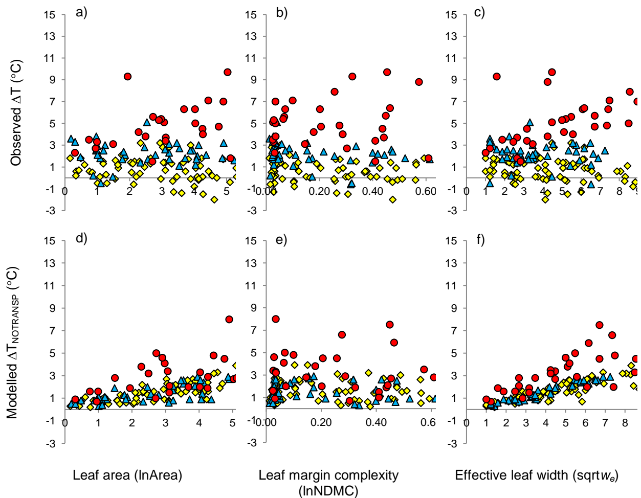
Figure 4. Comparison of the measured vs modelled leaf-to-air temperature difference ( \Delta T and \Delta T_{\text{NOTRANSPIR}} respectively) as a function of leaf area (a and d), margin complexity (NDMC, b and e) and effective leaf width ( w_e , c and f) for Proteaceae leaves. Observed \Delta T values (a-c) were based on the average leaf temperature across each leaf relative to ambient temperature at the time of measurement. Modelled \Delta T_{\text{NOTRANSPIR}} (d-f) used the same leaf and ambient parameters but assumed that leaves were not transpiring. Data are for leaves from three sampling seasons: winter (blue triangles), autumn (yellow diamonds) and summer (red circles). Data transformation and presentation as for Figure 3.
