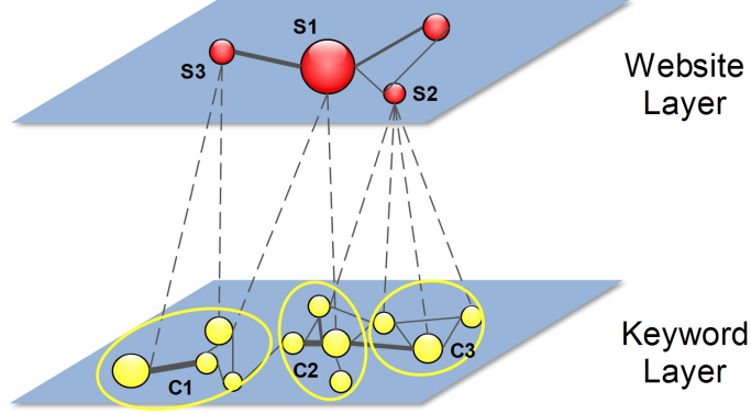
Figure 4: Intuitive method to discover the interests of websites. In this figure, there are three sample websites and related three communities in keyword layer network. It is the keywords that connect the communities with websites.
