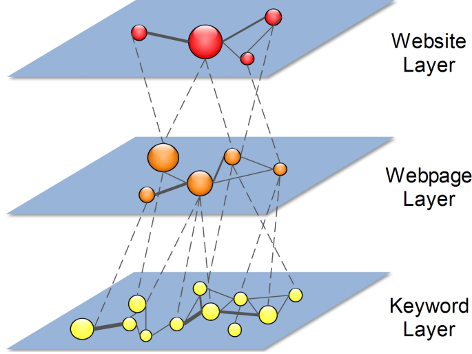
Figure 3: A three layered network for a news event e , comprising the website, webpage, and keyword layers. The red nodes in the top layer represent websites s , the orange nodes in the middle layer represents webpages p , and the yellow nodes in the bottom layer represent keywords k . A website may contain many webpages and a webpage may contain many keywords.
