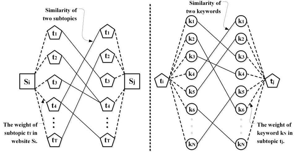
Figure 6: The evaluation metric used to compare the three methods. The left subfigure shows the similarity calculation between the interests of two websites, S_i and S_j , through their sub-topics. The right subfigure shows the similarity calculation between two sub-topics, t_i and t_j , through their keywords.
