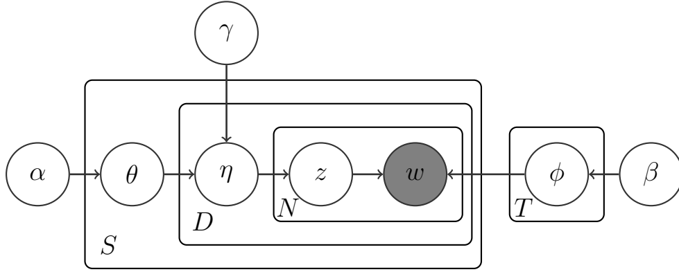
Figure 5: Graphical Models of website topic model
