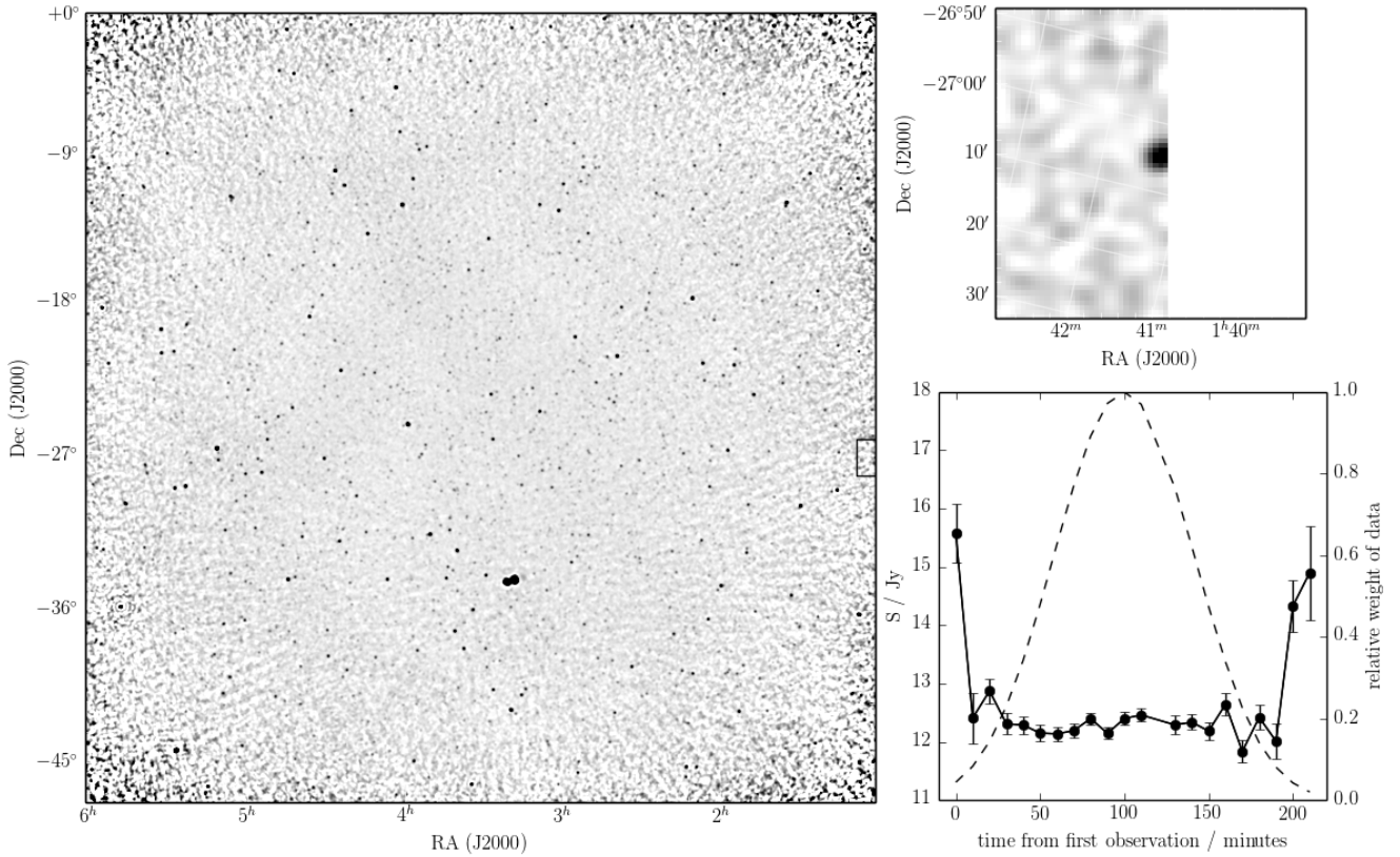
Figure 3. The left panel shows an animation, at four frames per second, of the central 45^\circ \times 45^\circ of the Dec-27 103–111 MHz drift data from the first twenty observations taken on the night of 2013 Nov 25, and following the imaging procedure outlined in Section 2.3.3. The central Dec remains constant throughout at Dec = -26^\circ 47' ; the first frame is centred on RA = 00^{\text{h}} 02^{\text{m}} and the last is centred on RA = 03^{\text{h}} 23^{\text{m}} . The greyscale is linear and runs from -0.1 – 1 \text{ Jy beam}^{-1} , and a primary beam correction has been made to produce a pseudo-Stokes-I view (not truly Stokes I, as the polarisation cross-terms are discarded, as described in Section 2.5). In order to enhance the visibility of the point sources in this figure, the images in this panel have been convolved with a Gaussian of FWHM 5' . A square indicates the area shown in the top right panel, which shows PKS J0141-2706 and the surrounding 45' \times 45' , with a linear grayscale from -1 – 10 \text{ Jy beam}^{-1} . The bottom right panel shows the measured integrated flux density of PKS J0141-2706 in each image (points; solid lines), with the local RMS of the image shown as an error bar. The dashed line shows the square of the primary beam response, which, combined with a global image RMS measurement, is the weighting given to each measurement at the mosaicking stage. NB: Due to size limits, the animation is only visible in the online version of this article. In printed versions, the last frame will display; note that in this frame, the test source is on the edge of the image, so while it is detected, its measured flux density is unreliable.
