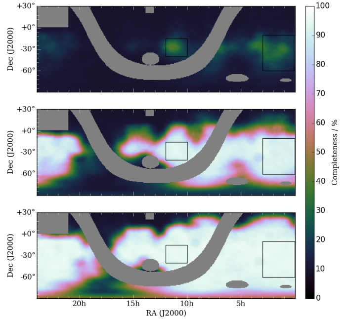
Figure 14. The top, middle and bottom panels show completeness maps at 25, 50 and 75 mJy, respectively, for the regions covered by the GLEAM catalogue of this paper. Areas which are excluded from the survey are shaded grey. The image projection used is Cartesian. The most sensitive areas of the survey in which the completeness was calculated in Figure 13 are outlined in black. FITS images of these completeness maps are available online.
