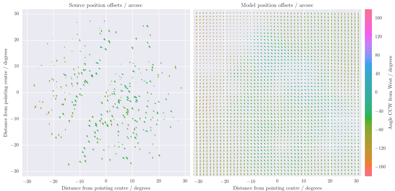
Figure 2. An animation, at four frames per second, of the measured and modelled ionospheric distortions for 44 observations performed on the night of 2013 Nov 25, at 72–80 MHz, where the distortions are largest. The left panel shows source position offsets, as measured by comparing the positions of 8\text{-}\sigma unresolved sources with the MRC and NVSS catalogues (see Section 2.4 for a full description of the cross-matching). The vectors indicate the direction of the correction that needs to be applied to align GLEAM with the reference catalogues. The right panel shows a radial basis function fit to these vectors, with values shown over a grid of 50 \times 50 points. In both panels, the axes are plotted in (l, m) rather than in equatorial co-ordinates. The diagonal gap in the source offset measurements in the last ten observations is caused by the Galactic Plane. In printed versions, only the last frame will display.
