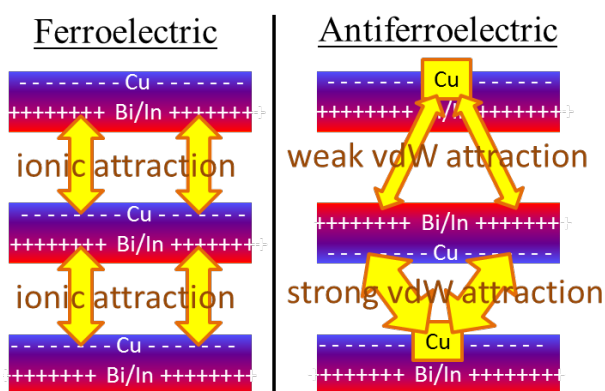
Fig. 4 The primary ionic and van der Waals (vdW) interactions between layers of ABP_2X_6 laminar materials. The ionic forces are weak but provide net stabilization of ferroelectric polymorphs compared to antiferroelectric ones, whereas the differences in inter-layer van der Waals interactions focus on the interaction of the Cu atoms with the electron-rich parts of the neighbouring bilayer, strongly stabilizing A_{ii} bilayers while destabilizing A_{oo} bilayers compared to ferroelectric ones.
