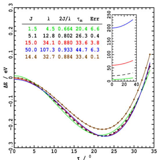
Fig. 5 The 1962 Swalen and Ibers 128 (black dots) and 2011 NH3-2010 Yurchenko et al. 130 (brown dots) adiabatic potentials g for the torsional motion ( \nu_2 ) of NH 3 are fitted up to 34° by various 3-state 3-parameter diabatic-potential models: black, brown dashed- all parameters optimized, else optimization with J constrained. The insert shows the associated double- excitation adiabatic surfaces whilst the tabulated diabatic potential parameters are J (eV), \lambda (eV) and \tau_m (°), while the RMS error in the fits is also given (meV).
