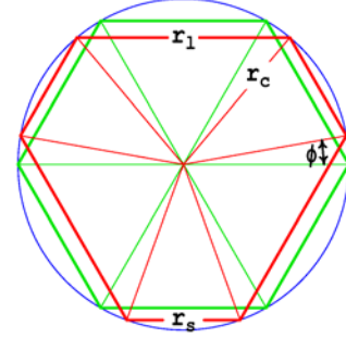
Fig. 9 Definition of the angle \phi (shown here at 10^\circ ) and the radius r_c (shown here angle independent for simplicity) used for the description of the {}^1\text{b}_{1u} Kekulé distortion of benzene, producing short and long CC bond lengths r_s and r_l , respectively.
