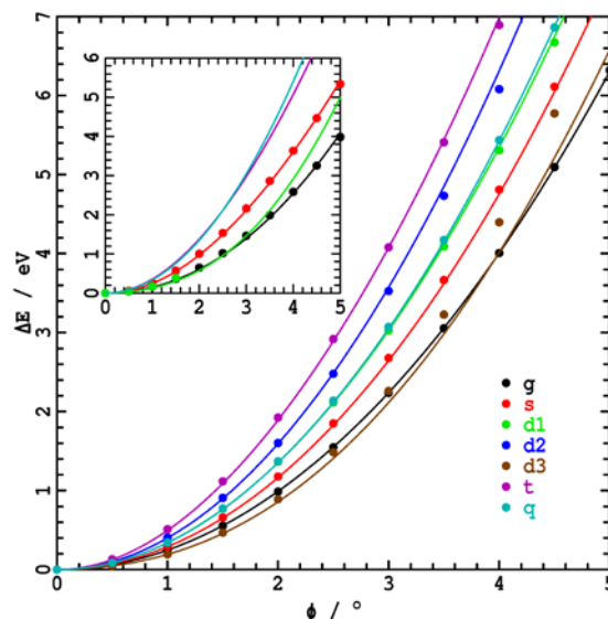
Fig. 11 Calculated (points) and diabatic-model fitted (lines) adiabatic potential-energy surfaces, expressed relative to the energy at the D 6h symmetric structure given in Table 4, for the various coupled HOMO→LUMO multiple excitations of benzene as a function of the Kekulé distortion angle \phi (see Figs. 2 and 8). The main plot shows results at the CAS(4,4)/6-31G* level whilst the insert shows those after second-order perturbation-theory correction, NEVPT2.
