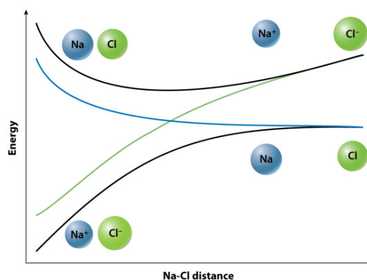
Fig. 1 Diabatic surfaces representing the \text{Na}^+\text{-Cl}^- (green) and \text{Na}\cdot\text{-Cl}\cdot (blue) chemical descriptions of the NaCl molecule are mixed to give ground-state and excited-state adiabatic potential-energy surfaces (black). As the molecule stretches, the adiabatic surfaces change character whilst the diabatic surface do not. Taken from van Voorhis et al., 2 reproduced with permission of Annual Reviews .
