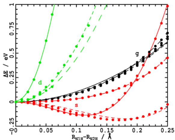
Fig. 8 Changes in adiabatic energies from those at the D_{3d} geometry for the g (black), s (red), and d (green) potential-energy surfaces of protonated ammonia dimer \text{N}_2\text{H}_7^+ as a function of the proton-transfer coordinate \Delta R = R_{\text{N1H}} - R_{\text{N2H}} , evaluated using the STO-3G basis by CAS(2,2) (solid lines), CAS(2,8) (short-dashed lines) and EOM-CCSD (long-dashed lines); points- raw calculated data, lines- adiabatic model fits to the data, see Table 3, (solid lines).
