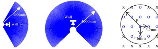
Fig. 2. a) Tilt Scan (Side view): Increments of 1/3^\circ ; b) Pan Scan (Top view): Increments of 0.36^\circ ; c) 3D Scan Points on wall at 1m range (within workspace ): distance between points (o=points within circle radius \mu ; x=points outside circle)
