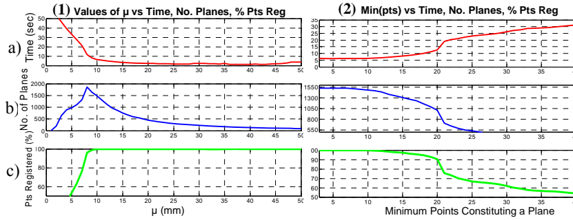
Fig. 5. (1) With respect to \mu(\text{mm}) (a) \Delta time; (b) No. of planes; (c) Points registered (%) (2) With respect to \text{min}(\text{pts}) ; (a) \Delta time; (b) No. of planes ; (c) Points registered (%)
