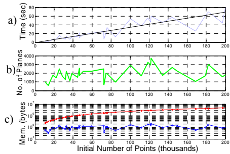
Fig. 8. Results for increasing No. of initial points; a) Overall time (grey) and the trend line (black); b) No. planes; c) Data reduction: original (red *) and post processing (blue o)
