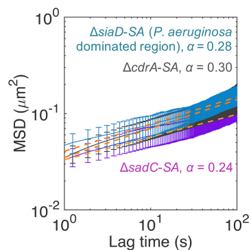
FIG 6 MSD curves for P. aeruginosa \Delta siaD - S. aureus , P. aeruginosa \Delta cdrA - S. aureus , and P. aeruginosa \Delta sadC - S. aureus microcolonies. SA, S. aureus . The orange dotted lines indicate the line of best fit to the experimentally determined MSD using a power law function for the estimation of \alpha . Error bars represent SEM.
