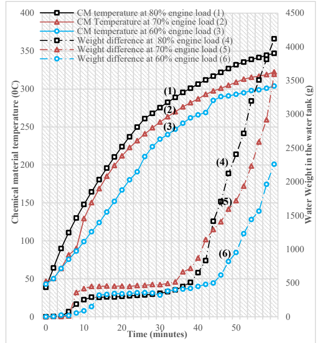
Figure 7: CM temperature ( T_3 ) and the water weight in the water tank in the heat storage process at 80%, 70% and 60% engine loads
