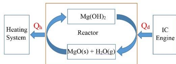
Figure 1: The principle of CHS system using EM8block to store exhaust gas energy of IC engine
