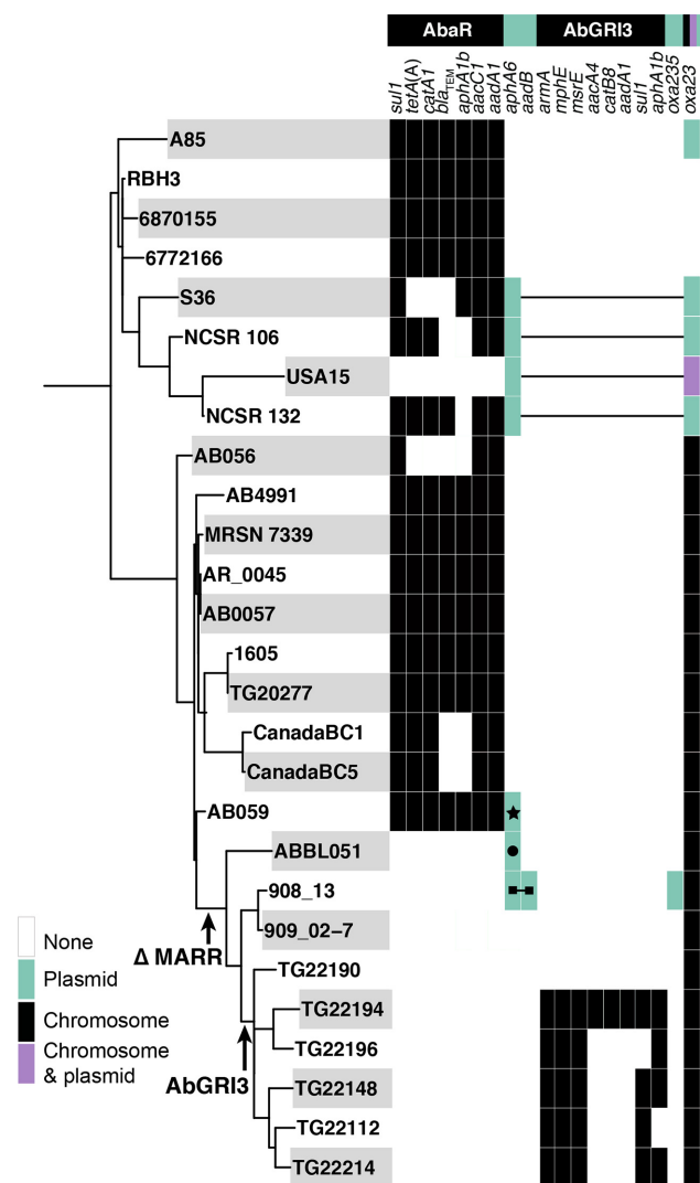
Fig. 4. Phylogenetic tree combined with the distribution of antibiotic-resistance genes. Black rectangles indicate resistance genes found in the chromosome, green rectangles represent plasmid-associated genes with symbols indicating different plasmids, and purple rectangles show genes found both in the chromosome and the plasmid in USA15. Antibiotic-resistance genes predicted to be in AbaR and AbGRI3 are separated and shown as two different blocks. The black lines, linking green/purple rectangles, indicate genes found on the same plasmid.
