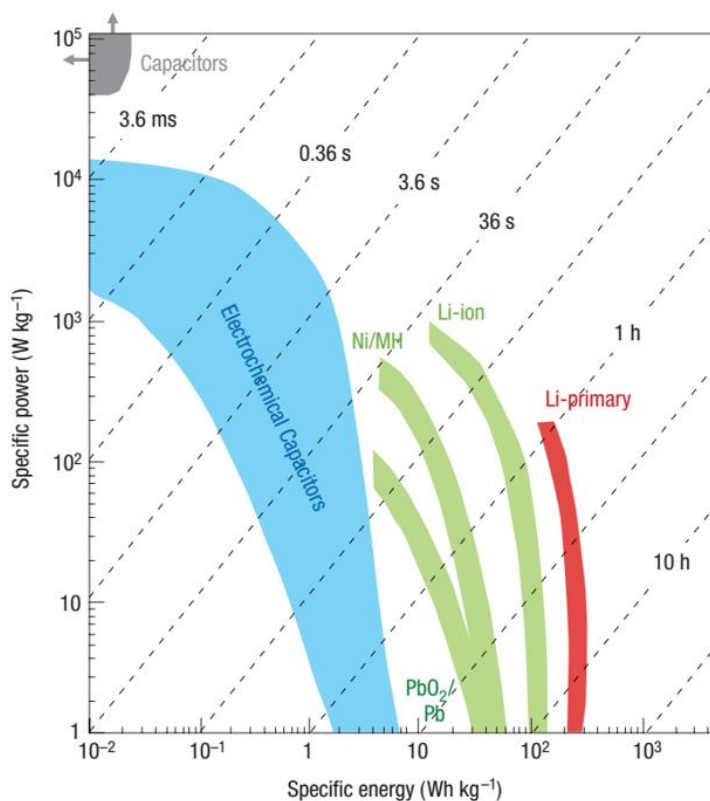
Figure 1 Ragone plot related to specific energy and power of typical electrochemical capacitors compared with other electrochemical energy storage systems. Reproduced with permission of the Nature Publishing Group. 52
