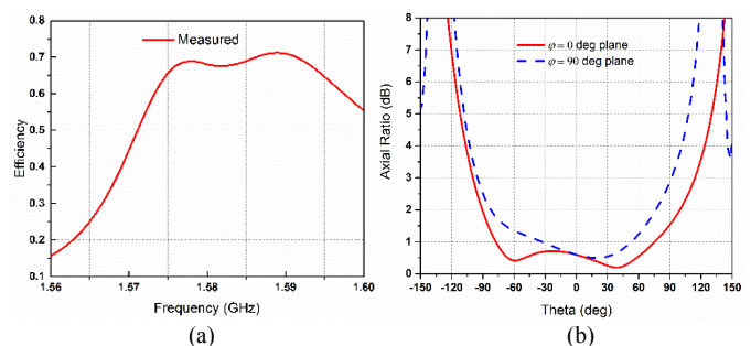
Fig. 11. Measured antenna parameters. (a) Total efficiency as functions of the source frequency. (b) AR beamwidth in the two vertical planes: \varphi = 0^\circ and \varphi = 90^\circ at 1.584 GHz.
