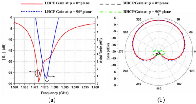
Fig. 5. Simulated results of the HCP ESA with the unbalanced crossed-dipole excitation structure. (a) |S_{11}| and AR values as functions of the source frequency. (b) The LHCP and RCHP realized gain patterns at 1.575 GHz.
