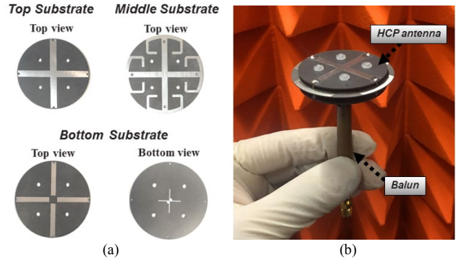
Fig. 8. HCP ESA. (a) Photos of the fabricated components. (b) The assembled prototype with a sleeve balun.
