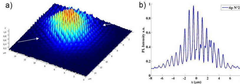
Fig. 8. a) Near-field intensity distribution of mode-M collected with tip N°2 at 1611 nm b) Mode section recorded along the direction of the white arrows of a), .
