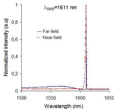
Fig. 3. Far-field and near-field spectra of honeycomb lattice normalized to the maximum intensity. Mode M at \lambda_{\text{SBM}} = 1611 nm matching well in two types of measurement.
