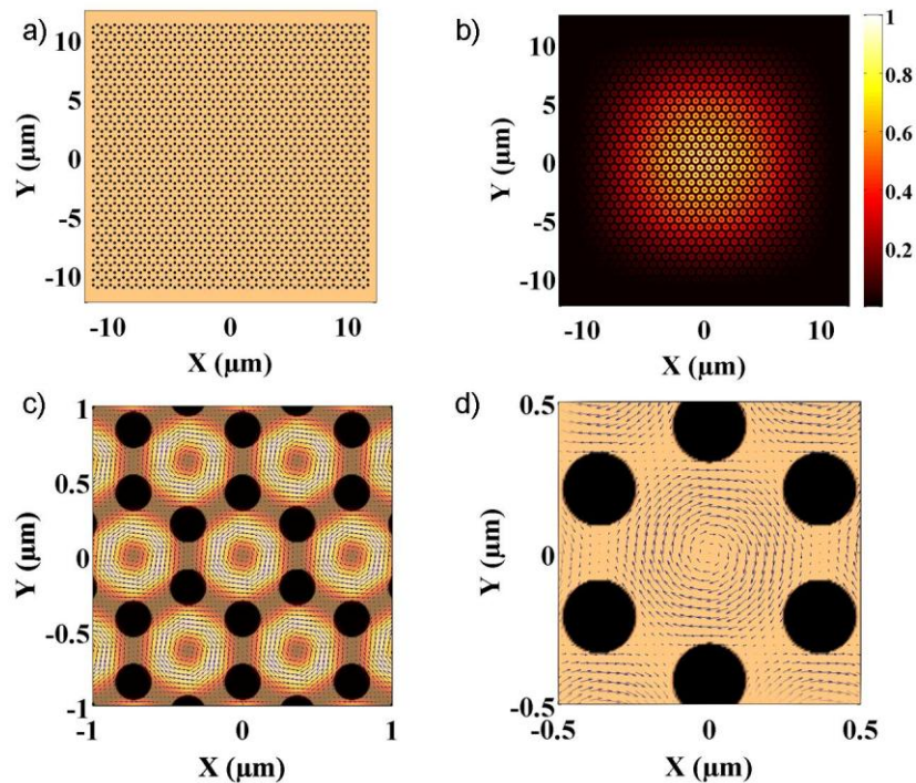
Fig. 1. 3D-FDTD simulation of the monopolar mode at the surface of a 2D-PC slab honeycomb structure. a) Overview of the PC structure. b) Normalized field intensity ( E_x^2 + E_y^2 ) at the surface of the PC at 1602 \text{ nm} . c) Zoom over the central part of the PC showing intensity map with the air holes in black, d) Electric field pattern illustrating the azimuthally polarized field in each unit cell.
