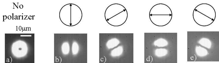
Fig. 4. Image of the mode at the surface of the PC in the far-field zone (the image is collected through a microscope objective with an NA of 0.75). a) Image of the mode without polarizer, b)-e) images with a polarizer oriented respectively at 0°, 60°, 90°, and 120°.
