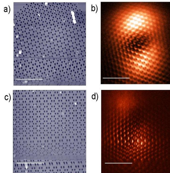
Fig. 6. a) Topography in shear-force mode with metallized tip N°1 b) Near-field distribution of intensity of mode-M recorded with tip N°1 at 1611 nm, the scaling bar is 5 \mu\text{m} , c) Topography with tip N°2, d) Near-field distribution of intensity of mode-M recorded with tip N°2 at 1611 nm, the scaling bar is 5 \mu\text{m}
