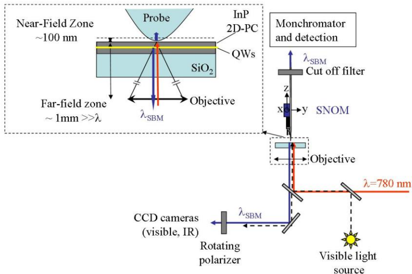
Fig. 2. Experimental set-up: near-field and far-field analysis are implemented.
