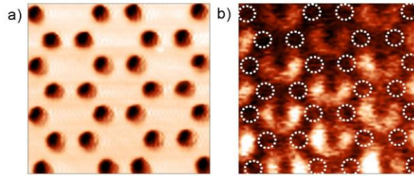
Fig. 7. Detail of the M-mode, a) Topographic image b) Optical near-field image at 1611 nm ( 2.5\mu\text{m} \times 2.5\mu\text{m} ), circles indicate holes positions of the 2D-PC. In one unit cell, the outer radius of the doughnut is 310 nm and the inner radius 70 nm ( \lambda/10 ).
