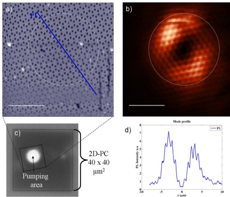
Fig. 5. a) Topography in shear-force mode b) Near-field distribution of intensity of mode-M recorded with a bare silica tip at 1611 nm, the scaling bar is 5 \mu\text{m} , c) CCD image in the visible range of the excitation spot (780 nm) on the structure, the width of the gaussian beam is about 9.5 \mu\text{m} , d) Mode section recorded along the line P1 (corresponding to \Gamma\text{K} direction in the reciprocal space)
