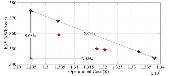
Fig. 7. Two-dimension Pareto front for operational cost-ENS
