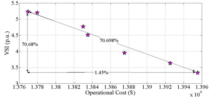
Fig. 8. Two-dimension Pareto front for operational cost-VSI
