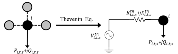
Fig. 1. Thevenin equivalent system of bus i at t^{th} hour for s^{th} scenario
