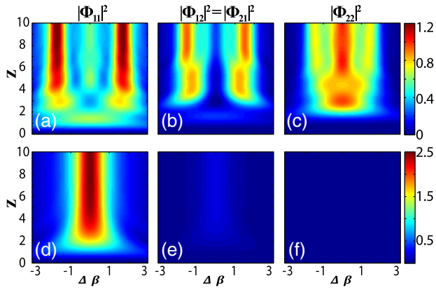
Fig. 2. Evolution of spatial signal and idler photon correlations between the two waveguide modes along the propagation direction ( z ) depending on the phase mismatch ( \Delta\beta ) for different losses in the second waveguide \gamma_s = \gamma_i = \gamma . (a)–(c) \gamma = 0.5 below the PT-symmetry breaking threshold. (d)–(f) \gamma = 3 corresponding to PT-broken regime. For all plots, the coupling coefficients are C_s = C_i = 1 , C_p = 0 , and pump is coupled to the first waveguide, A_1(z=0) = 1 , A_2(z=0) = 0 , and \gamma_p = 0 .
