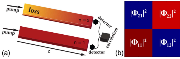
Fig. 1. (a) Scheme of generation of photon pairs through the spontaneous parametric down-conversion in a nonlinear PT-symmetric coupler with linear absorption in the second waveguide. (b) Graphical representation of biphoton correlation function |\Phi_{n_s, n_i}|^2 .
