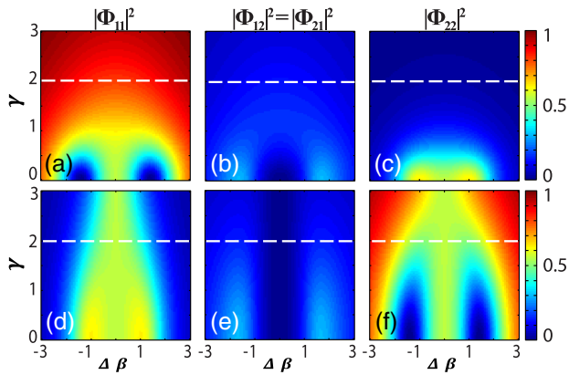
Fig. 3. Normalized photon correlations, |\Phi_{n_s, n_i}|^2 / \sum_{n'_s, n'_i} |\Phi_{n'_s, n'_i}|^2 , versus the phase mismatch and loss in the second waveguide at the fixed propagation distance z = 10 . The pump is input to the (a)–(c) first [ A_1(z=0) = 1 , A_2(z=0) = 0 ] or (d)–(f) second waveguide [ A_1(z=0) = 0 , A_2(z=0) = 1 ]. Dashed lines indicate the linear PT-breaking threshold at \gamma_{PT} = 2C . Other parameters correspond to Fig. 2.
