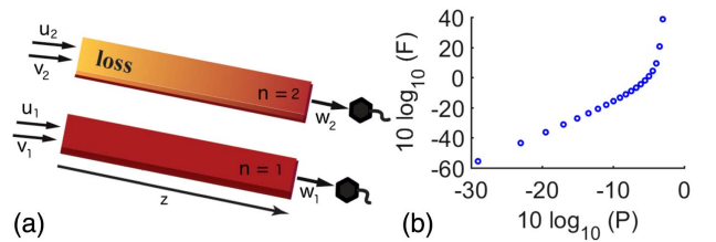
Fig. 4. (a) Scheme of SFG in passive PT-symmetric nonlinear coupler with linear absorption in one waveguide. (b) Mismatch F between the SPDC and SFG depending on the input power P for |u_{n_s}(z=0)|^2 = |v_{n_i}(z=0)|^2 = P/2 , plotted on a logarithmic scale. The propagation distance is z = 10 , signal and idler losses are equal \gamma_s = \gamma_i = 0.5 , there is no loss in the pump mode \gamma_p = 0 , and the coupling coefficients are C_s = C_i = 1 , C_p = 0 .
