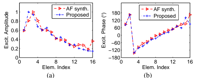
Fig. 4. The synthesized excitation distributions (corresponding to the patterns in Fig. 3) by the proposed method and the method in [1]. (a) Excitation amplitudes, and (b) excitation phases.
