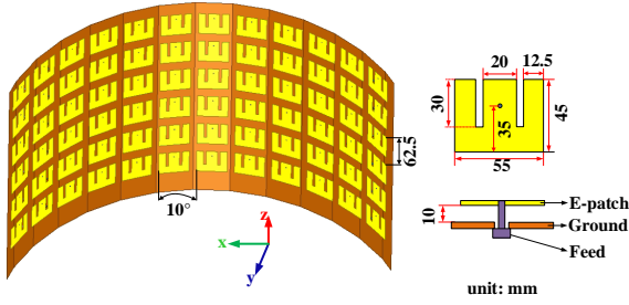
Fig. 9. Geometry of a cylindrical array with 12 \times 6 E-type patch antennas.
