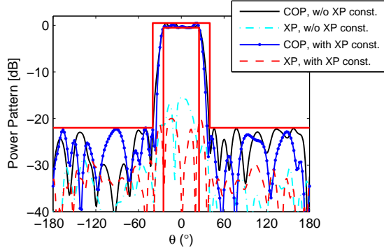
Fig. 6. The obtained COP and XP patterns for the sectorial array by the proposed method with/without a -20 dB XPL constraint.
