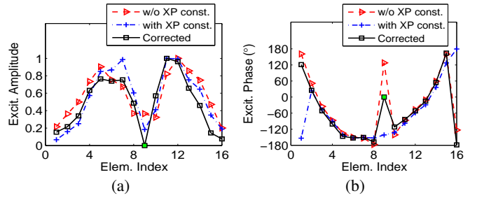
Fig. 8. The synthesized excitation distributions by the proposed method with/without XPL constraint as well as the corrected excitations for the damaged array (the 9th element is not excited). (a) Excitation amplitudes, and (b) excitation phases.
