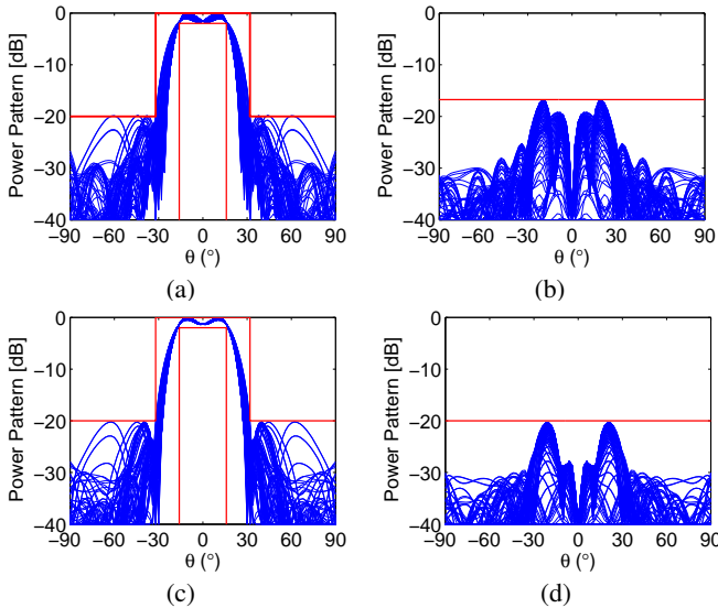
Fig. 11. The \varphi -cuts (in step of 1^\circ ) of the synthesized circular flat-top patterns for the 12 \times 6 -element cylindrical array by the proposed method. (a) The COP pattern without XPL constraint, (b) the XP pattern without XPL constraint, (c) the COP pattern with a -20 dB XPL constraint, and (d) the XP pattern with a -20 dB XPL constraint.
