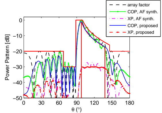
Fig. 3. The synthesized COP and XP patterns for the linear array by the proposed method with accurate vectorial pattern control and the array factor synthesis method in [1].
