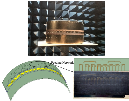
Fig. 13. The fabricated 16-element sectorial conformal array with the feeding network on the reverse side of the ground.
