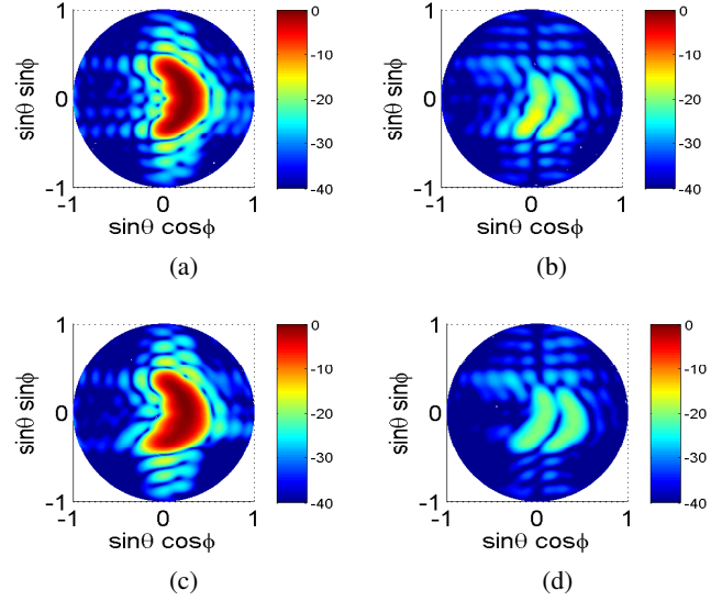
Fig. 12. Top views of the synthesized crescent-shaped patterns for the 12 \times 12 -element cylindrical array by the proposed method. (a) The COP pattern without XPL constraint, (b) The XP pattern without XPL constraint, (c) the COP pattern with a -20 dB XPL constraint, and (d) the XP pattern with a -20 dB XPL constraint.
