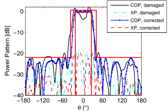
Fig. 7. The obtained COP and XP patterns of the damaged sectorial array (the 9th element is not excited) and the corrected COP and XP patterns by re-optimizing the excitations of the left elements.
