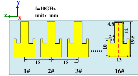
Fig. 2. Geometry of a 16-element microstrip antenna array (a substrate with \epsilon_r = 2.2 and thickness of 1.57 mm is used).
