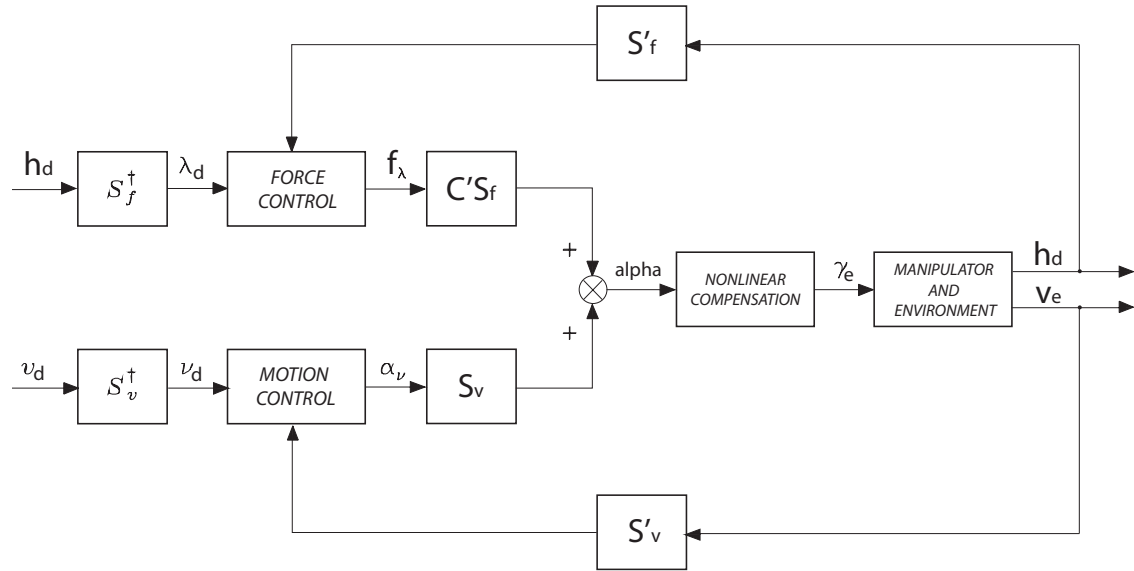
Fig. 2. Block scheme of a hybrid force/motion control for a compliant environment
