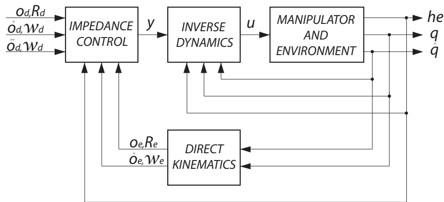
Fig. 1. Block scheme of impedance control
