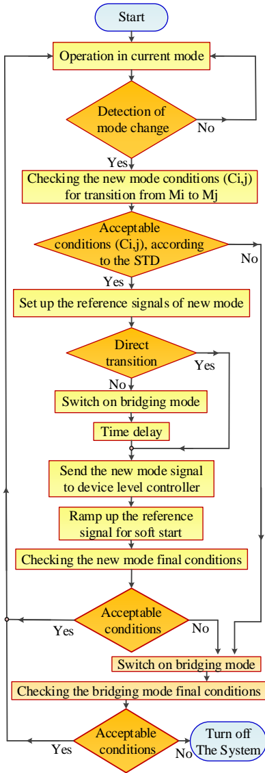
Fig.14. Flowchart of mode transition unit (MTU) operation
