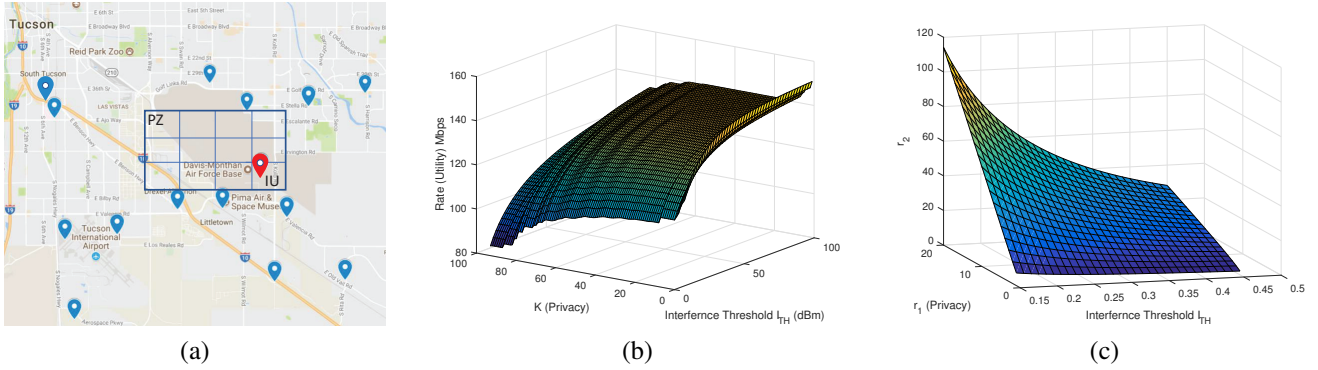
Figure 7: (a) Topology of a real-world deployment, (b) DOL: the three-way tradeoff, (c) POL: the three-way tradeoff.
