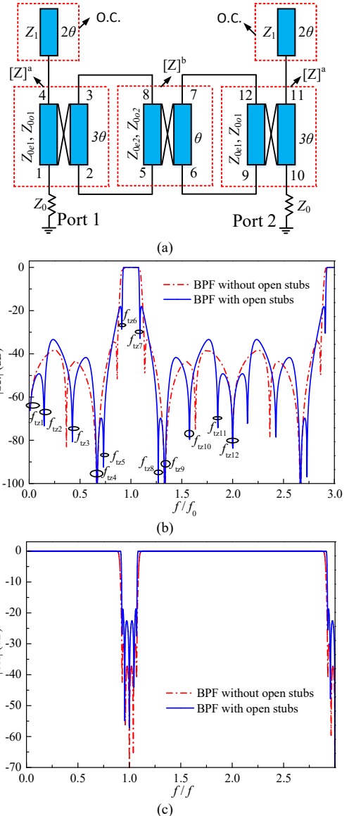
Fig. 1. (a) Ideal circuit, (b) simulated |S_{21}| and (c) |S_{11}| of the proposed BPF with \theta=90^\circ , Z_1=90 \Omega , Z_{0e1}=158 \Omega , Z_{0o1}=60 \Omega , Z_{0e2}=109 \Omega , Z_{0o2}=68 \Omega ( Z_{0o2}=65 \Omega when BPF without open stubs).
