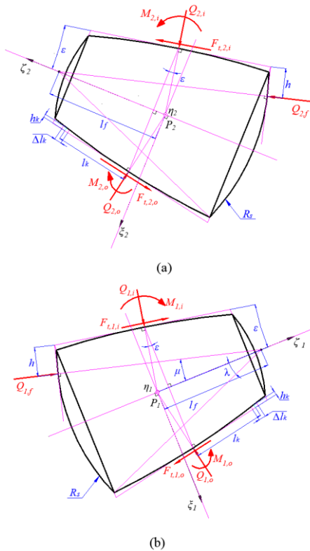
Fig. 3. Free body diagram of rollers: (a) a roller in row 2; (b) a roller in row 1.
