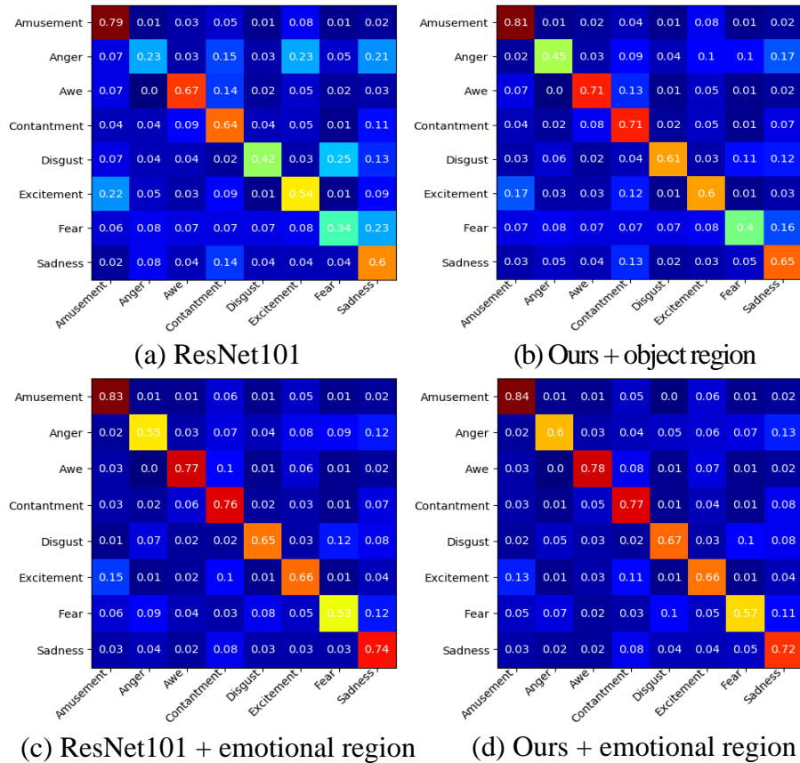
Figure 6: Confusion matrix for our method with different configurations and ResNet101.
