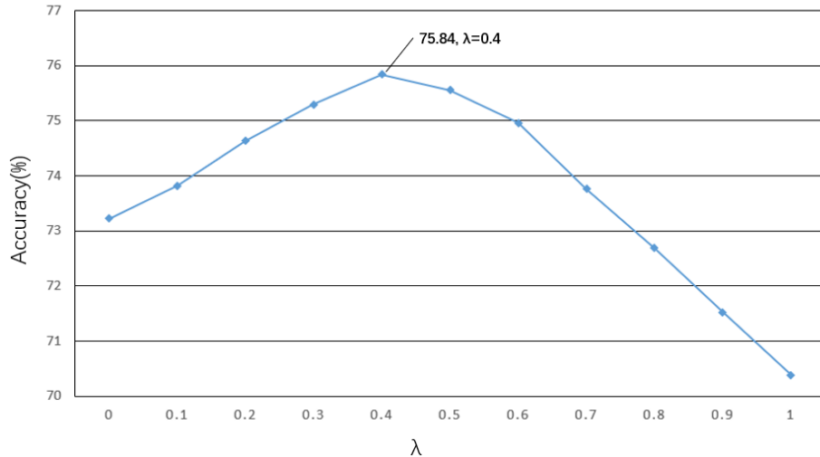
Figure 8: Impact of different \lambda on the validation set of the FI dataset. \lambda = 0.4 achieves the best performance and we choose it in all our experiments.
