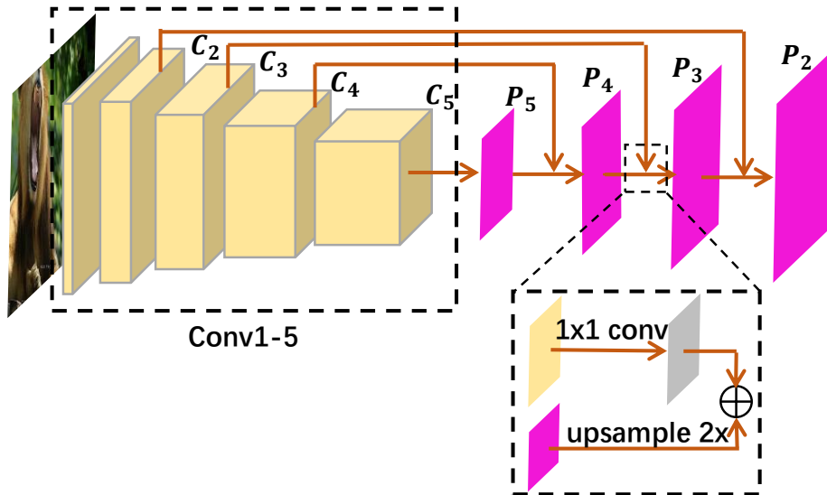
Figure 3: Structure of Feature Pyramid Network (FPN).
