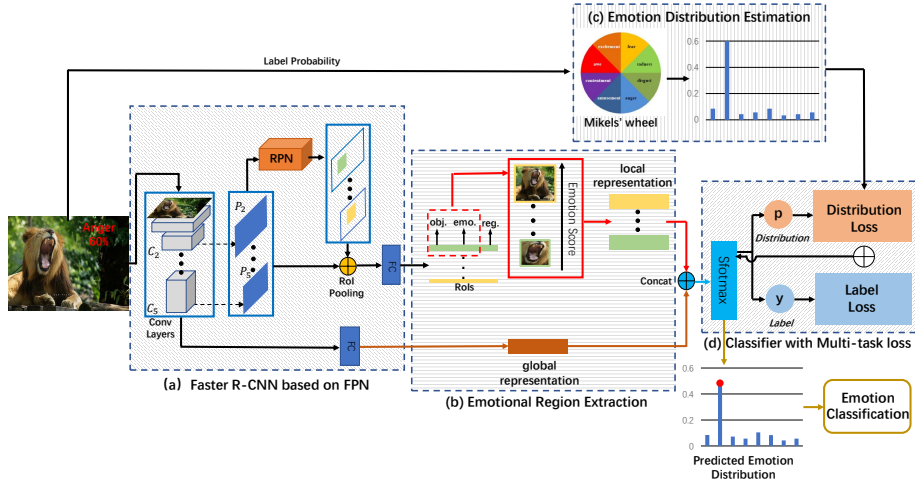
Figure 2: The overview of the proposed framework. The framework consists 4 components:(a) faster R-CNN based on FPN, (b) emotional region extraction based, (c) emotion distribution estimation and (d) classifier with multi-task loss.
