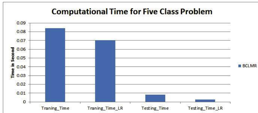
Figure 8: Computational Time for Five-Class Problem.
