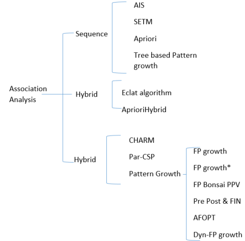
Fig. 3. Association Mining Methodologies
