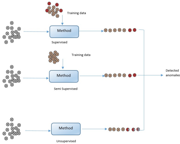
Fig. 4. Anomaly detection methods based on dataset
