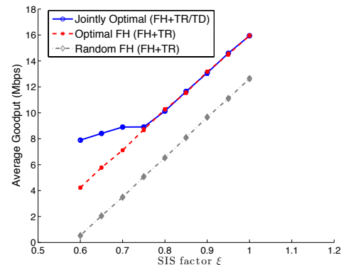
Fig. 19: Avg. goodput vs. \xi
