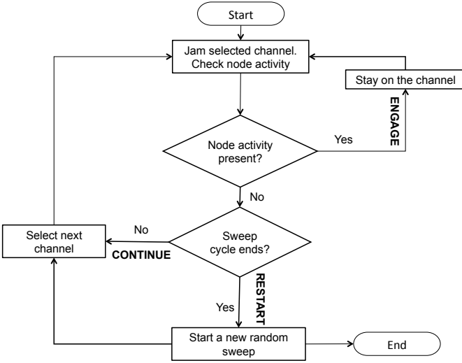
Fig. 2: IBFD Reactive Sweep Jammer : In each time slot, the jammer attacks one selected channel and observes channel activity. If some activity is observed, it stays on the channel and continuously attacks it (ENGAGE state). Otherwise, it RESTARTs a new sweep pattern if this is the end of the current cycle, else it attacks the next channel in the sweep cycle (CONTINUE state).
