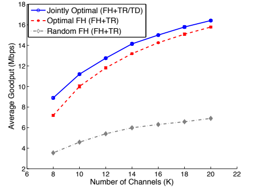
Fig. 10: Avg. goodput vs. K
