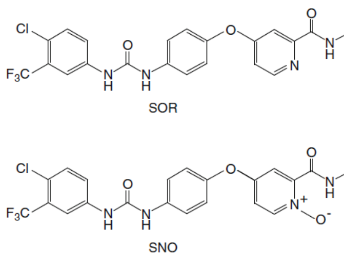
Fig. 1. Structures of SOR and its major metabolite SNO
