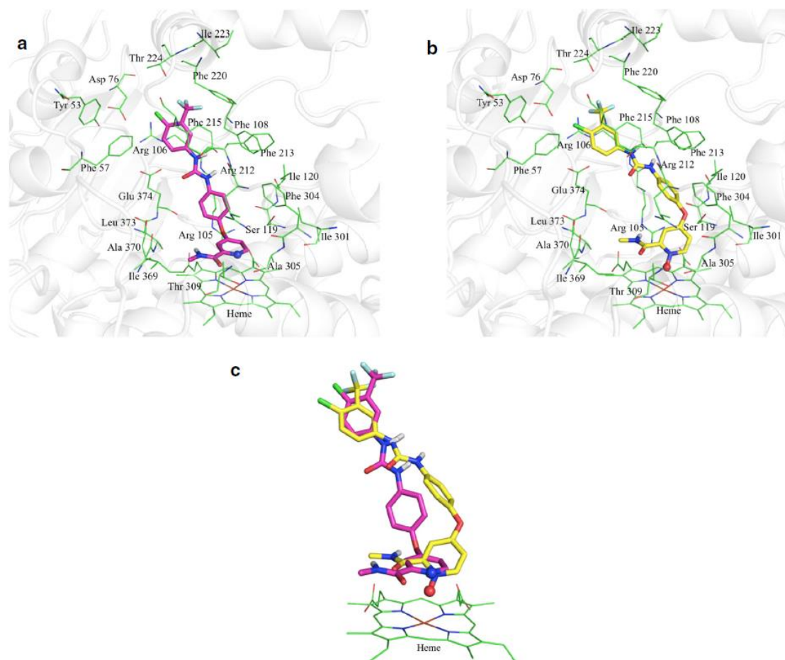
Fig. 6. Docked poses of SOR and SNO in the catalytic site of CYP3A4. a SOR, b SNO, and c overlay of SOR and SNO. Key amino acid residues involved in binding interactions are numbered
