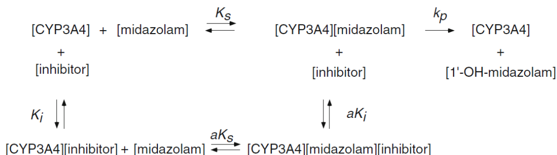
Fig. 5. Michaelis–Menten equilibria showing CYP3A4-inhibitor/substrate complex formation and linear mixed-type reversible inhibition of CYP3A4-dependent midazolam 1'-hydroxylation. [inhibitor] refers to either SOR or SNO (as shown in Figs. 3 and 4, respectively).
