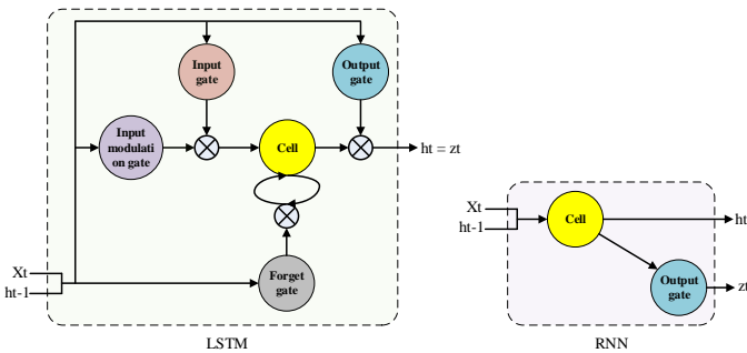
Fig. 7: An illustration of a basic (a) LSTM and (b) RNN cell.
