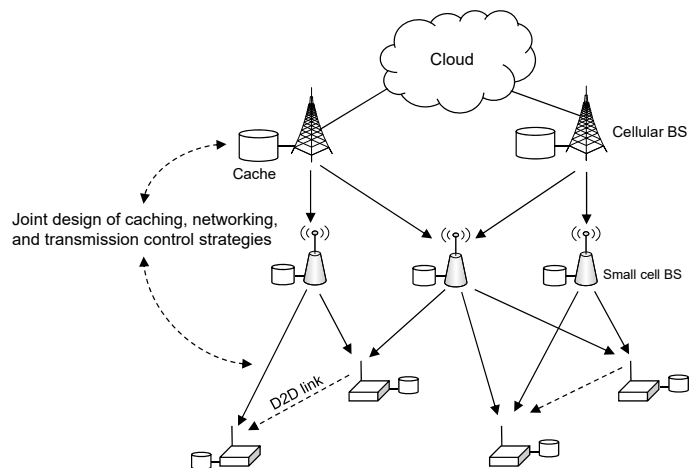
Fig. 15: Joint caching, networking, and transmission control to optimize cache hit rate [78], cache expiration time [82], interference alignment [85]–[87], Quality of Experience [88], [90], energy efficiency [93], resource allocation [94]–[96], traffic latency, or redundancy [98], [100].
