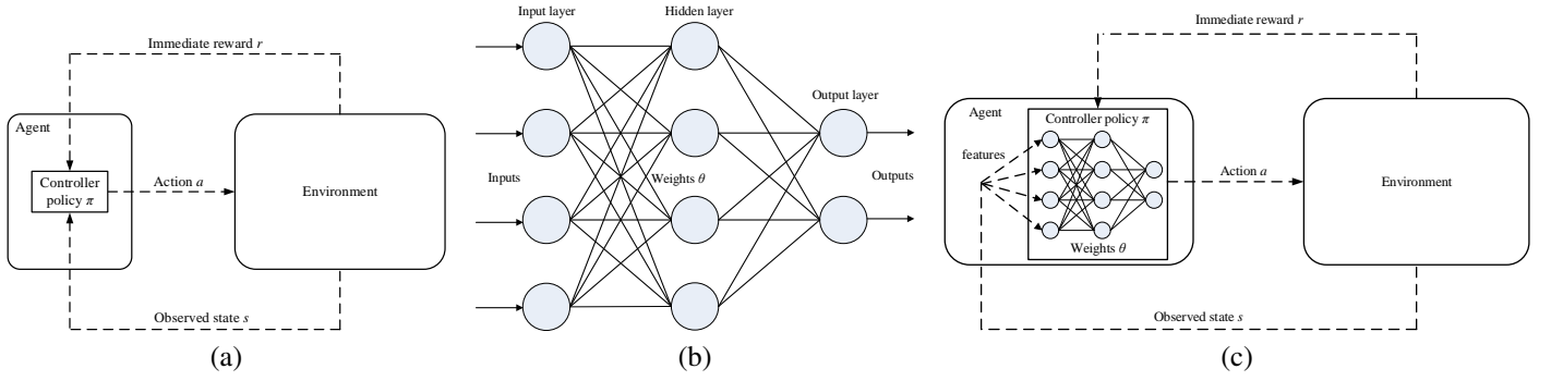
Fig. 4: (a) Reinforcement learning, (b) Artificial neural network, and (c) Deep Q-learning.
