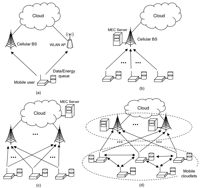
Fig. 16: Data/computation offloading models in cellular networks: (a) Offloading cellular traffic to WLAN [103], (b) Offloading to a single MEC-enabled BS [104], (c) Offloading to one shared MEC server via multiple BSs [105], [106], [110], (d) Offloading to multiple MEC-enabled BSs [114], [115] and mobile cloudlets [116], [117].
