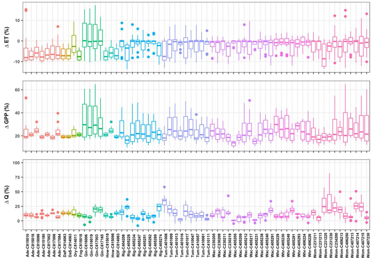
Figure 3-6. Variation in multi-year average monthly Q, ET, and GPP in response to increased atmospheric CO 2 concentration. CO 2 increase by 45% (from 380 ppm to 550 ppm). For all three variables, simulated values with the 380 ppm CO 2 concentration were used as benchmark. Variation was calculated as the difference between simulated values under 380 ppm and those under 550 ppm (Eq. 3-6). The solid line in each box represents the median value, whiskers are the 5 th and 95 th percentiles, solid circles represents outliers. The 25 th and 75 th percentiles are shown as the lower and upper boundaries of each box.
