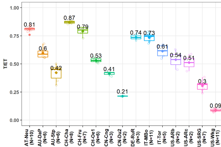
Figure 4-2. Multiyear average T/ET estimates by the PML_V2 model. N represents the number of years used at each study site. The mean (solid diamond (number in black)) and median (horizontal line) values are shown in each box. Values for individual site-years are shown as circles, and the 25 th and 75 th percentiles are shown as the lower and upper boundaries of each box. Whiskers represent the 5 th and 95 th percentiles.
