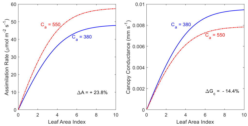
Figure 3-5. Sensitivity of carbon assimilation rate and canopy conductance to increased in atmospheric CO_2 concentration. C_a = 380 (ppm, or \mu\text{mol mol}^{-1} ) was set as the benchmark, C_a = 550 \mu\text{mol mol}^{-1} was the eCO_2 scenario. Environmental variables were given as P_a = 90 \text{ kPa} , R_s = 500 \text{ W m}^{-2} , PAR was set as 0.45 of R_s , T_{air} = 25^\circ \text{C} , VPD = 3 \text{ kPa} . Parameters were D_0 = 0.7 \text{ kPa} , \alpha = 0.103 , \eta = 0.04 , k_Q = 0.6 , m = 9 , A_{m,25} = 100 \mu\text{mol m}^{-2} \text{s}^{-1} . CO_2 was prescribed to increase by 45% (380 ppm set as benchmark elevated to 550 ppm). Variation in assimilation rate and canopy conductance was calculated according to Eq. 3-6.
