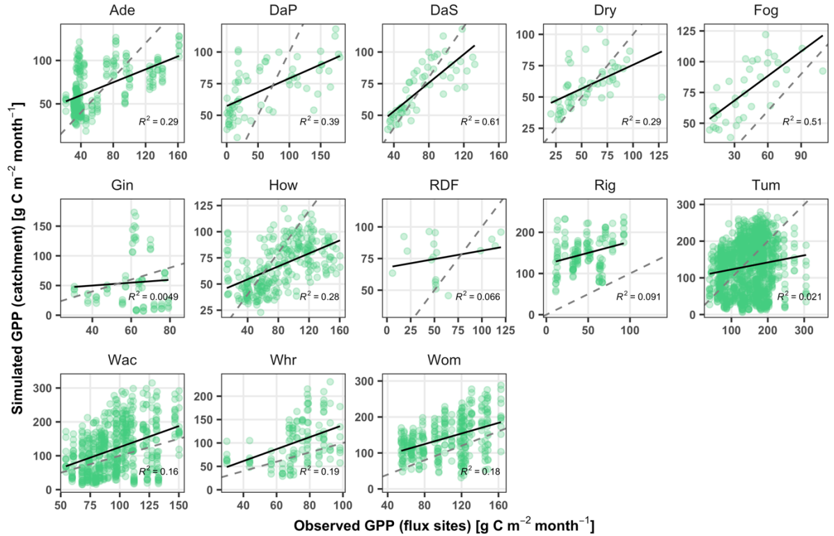
Figure 3-4.3. Simulated monthly gross primary production (GPP g C m -2 month -1 ) grouped by adjacent flux sites for 63 Australian catchments. The reference 1:1 line (dashed grey) and the linear regression line ( y = ax+b , solid black) are shown for comparison.
