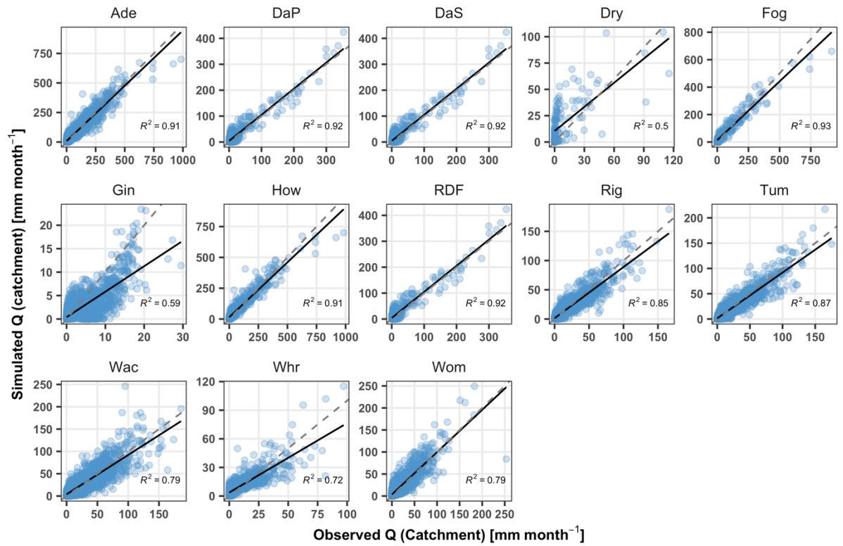
Figure 3-4.1. Simulated monthly catchment streamflow ( Q , \text{mm month}^{-1} ) vs observed streamflow grouped by adjacent flux sites for 63 Australian catchments. The reference 1:1 line (dashed grey) and the linear regression line ( y = ax+b , solid black) are shown for comparison.
