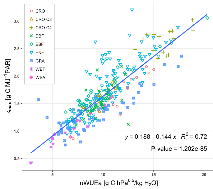
Figure S5-4. Relationship between the estimated \epsilon_{max} and the underlying water use efficiency ( uWUE_a = \text{GPP} \cdot \text{VPD}^{0.5} / \text{ET} ) across biome types. Biome types grouped and colored by plant functional type as in Figure S5-1.
