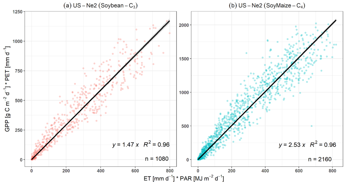
Figure 5-1. Comparison of \varepsilon_{max} estimates for C 3 and C 4 species at US-Ne2 (soybean grown in Nebraska, USA in 2002, 2004, 2006, and 2008 and maize grown in all other years) based on hourly observations during 2001-2012. The \varepsilon_{max} was estimated to be 1.47 g C MJ -1 PAR for C 3 (soybean) and 2.53 g C MJ -1 PAR for C 4 (maize) based on linear regression forced through the origin. ‘n’ represents the number of available hourly observations at this site.
