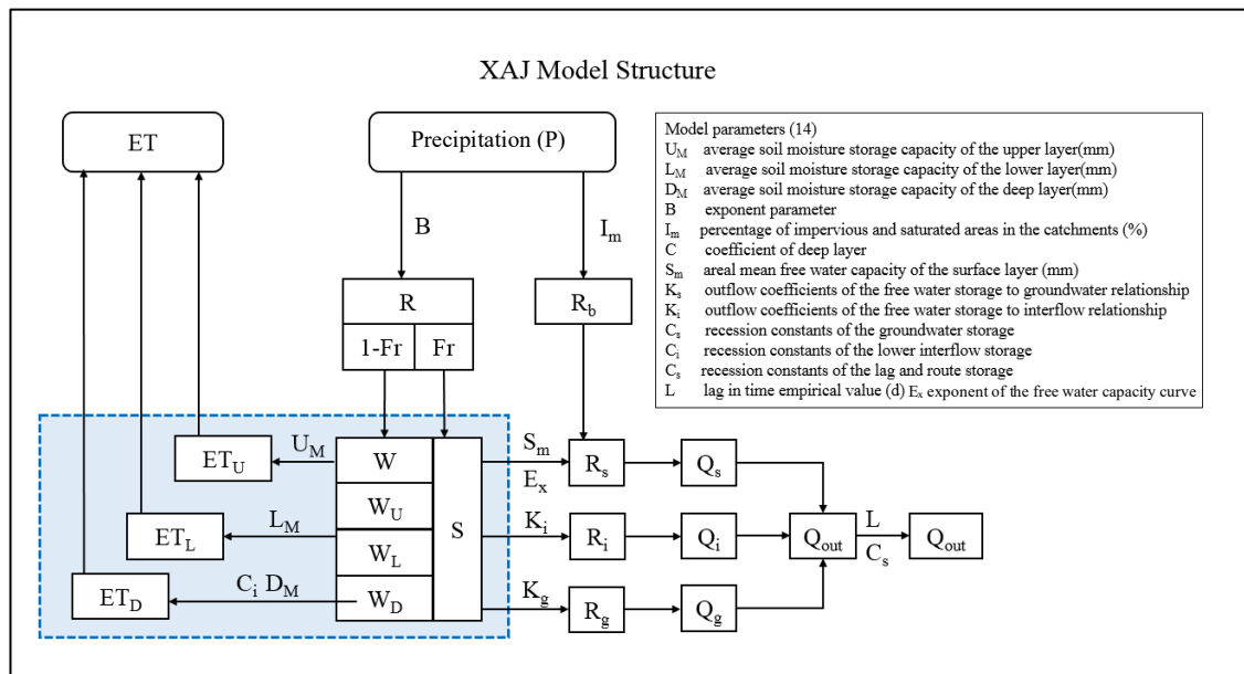
Figure 3-1. The Xinanjiang (XAJ) model structure, water storages (in boxes), and parameters (on arrow lines). The evapotranspiration sub-model is highlighted in the blue box, which will be revised later to align with the objectives of this study.
