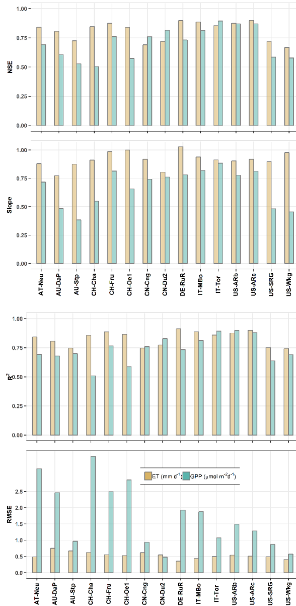
Figure 4-1. Statistics of model performance for 8-day time scale simulated ET and GPP. The model was optimised independently at each site based on available data. Nash-Sutcliffe efficiency (NSE), coefficient of determination ( R^2 ), linear regression slope (Slope) and RMSE (Root Mean Square Error) values were based on simulated versus observed data for both ET (yellow) and GPP (green).
