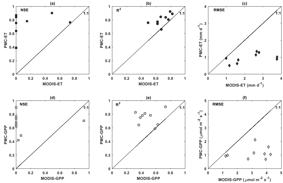
Figure 2-7. Statistic comparison of PML_V2 model (in validation mode) and MODIS products at nine Australian flux sites. NSE, R^2 and RMSE are given for ET (a-c) as black and GPP (d-f) as shaded symbols, respectively. The negative NSE values of MODIS products in (a) and (d) are set to zero to indicate low performance.
