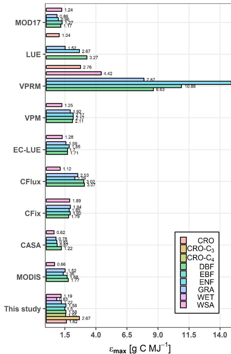
Figure S5-3. WUE-based \epsilon_{max} estimates from this study compared with different LUE-based modelling approaches across ecosystems. MOD17: look-up-table based on PFT from Running and Zhao 2015. LUE: a LUE model optimized at China flux sites from Wang et al. (2010). Other models optimized at 156 global flux sites from Yuan et al. (2014): CASA: Carnegie–Ames–Stanford Approach; CFix: Carbon Fix; CFlux: Carbon Flux; EC-LUE: Eddy Covariance-Light Use Efficiency; MODIS-GPP: Moderate Resolution Imaging Spectroradiometer GPP algorithm; VPM: Vegetation Production Model; VPRM: Vegetation Production and Respiration Model. Biome types grouped and colored by PFT following the same as Figure S5-1.
