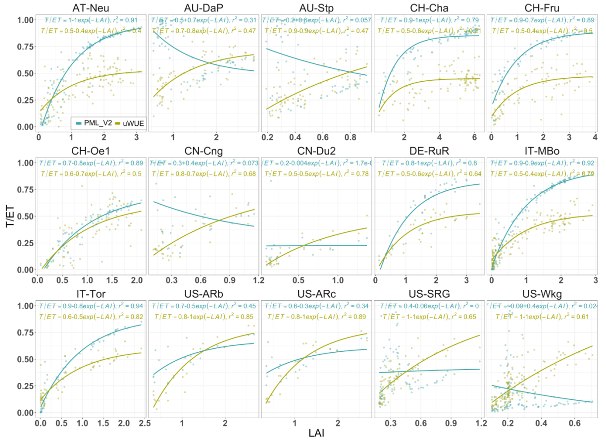
Figure 4-4. Relationship between monthly LAI and T/ET from the PML_V2 model (turquoise) and the uWUE (yellow green) method for each of the 15 flux sites. The natural exponential regression was performed between LAI and T/ET based on the two ET partitioning algorithms, with the fitted equation and R^2 shown accordingly.
