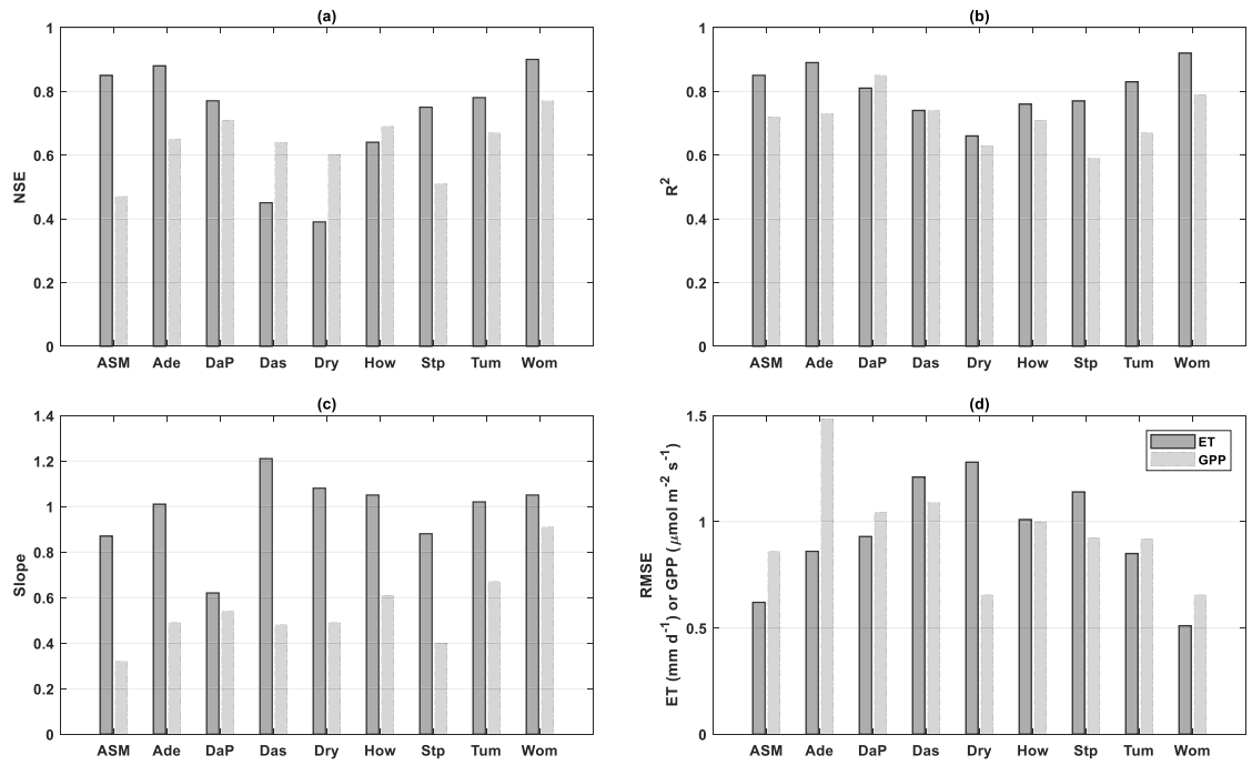
Figure 2-3. Statistics of model performance at 8-day time scale for ET and GPP estimates. The parameters are derived from independent optimisation using all available data at each site. Nash-Sutcliffe efficiency (NSE), coefficient of determination ( R^2 ), linear regression slope and RMSE, root mean square error of simulation against observation for both ET and GPP are presented.
