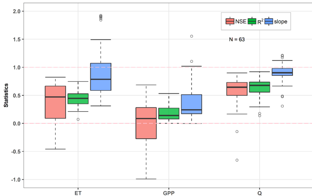
Figure 3-3. Summary of XAJ-PML_V2 model performance for streamflow (Q), evapotranspiration (ET), and gross primary production (GPP) across 63 (N) Australian catchments. The model was calibrated against observed daily Q at the catchment scale only. Simulated ET and GPP were compared with observed ET and GPP from adjacent eddy covariance flux sites near these catchments. Nash-Sutcliffe Efficiency (NSE), coefficient of determination ( R^2 ), and linear regression slope (slope) are shown across 63 catchments. The solid line in each box represents the median value, whiskers are the 5 th and 95 th percentiles, open circles represents outliers. The 25 th and 75 th percentiles are shown as the lower and upper boundaries of each box.
