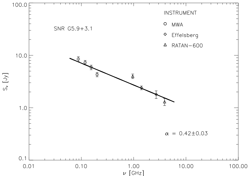
Fig. 2. Weighted least-squares fit of the presently known integrated radio continuum spectrum of the SNR G5.9+3.1 using the simple power-law model (Eq. 1) for pure synchrotron emission (solid line). Circles correspond to the MWA data, diamond symbols indicate Effelsberg data, and triangles depict RATAN observations.
