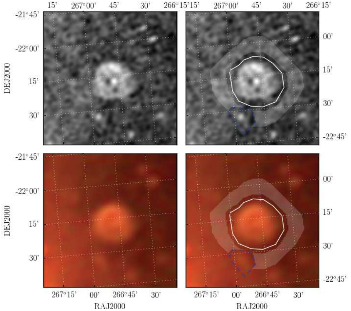
Fig. 1. GLEAM images of G5.9+3.1; the top two panels show the wideband image taken over 170–231 MHz, while the lower two panels show an RGB image comprised of R= 72–103 MHz, G= 103–134 MHz, B= 139–170 MHz. The full width at half maximums (FWHMs) of the point spread functions (PSFs) of the images are, respectively: 2.4', 5.2', 3.9', and 2.9'. The left panels show the images without any annotations. The right panels show annotations indicating the GLEAM photometry measurement: the white lines show the region drawn by the observer that contains the SNR; the gray shaded region shows the area used to calculate the background; the blue dashed lines show a region excluded from the background measurement for containing contaminating background radio galaxies.
