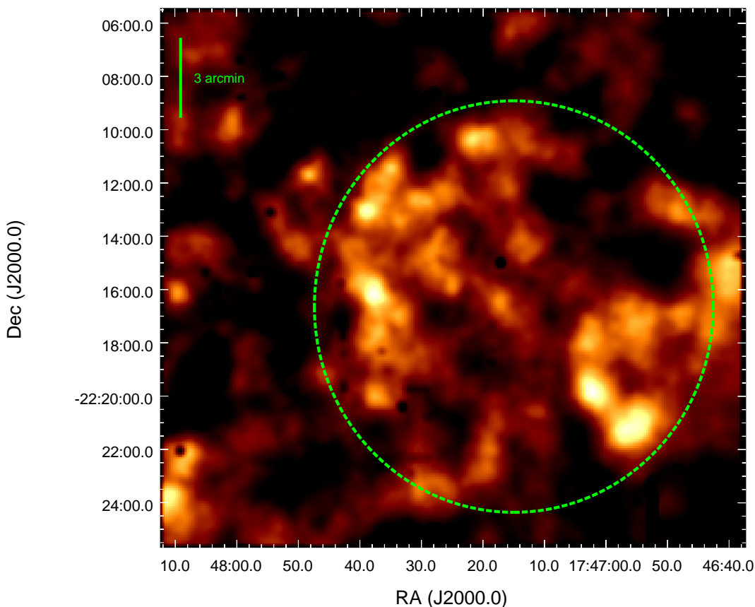
Fig. 3. Adaptively smoothed exposure-corrected combined EPIC image of G5.9+3.1. The image depicts emission detected over the energy range 0.4 keV to 1.0 keV and the pixel range of the emission is 3 to 7.87 counts per second per square degree. The dashed green ellipse is centered on RA (J2000.0) 17^{\text{h}} 47^{\text{m}} 15.0^{\text{s}} , Dec (J2000.0) -22^{\circ} 16' 38.5'' and has major and minor axes of 449.5'' and 463.4'' , respectively. This ellipse corresponds to the region of extraction of the source spectrum for the whole SNR (see Sect. 5 and Table 2). We note the clear rim-brightened structure seen toward the eastern and southwestern rims of G5.9+3.1. Fainter emission is seen toward the northern rim and interior of the SNR. Emission from discrete sources has been flagged and excised in the creation of this image: voids of emission seen in this image correspond to artifacts from these excisions.
