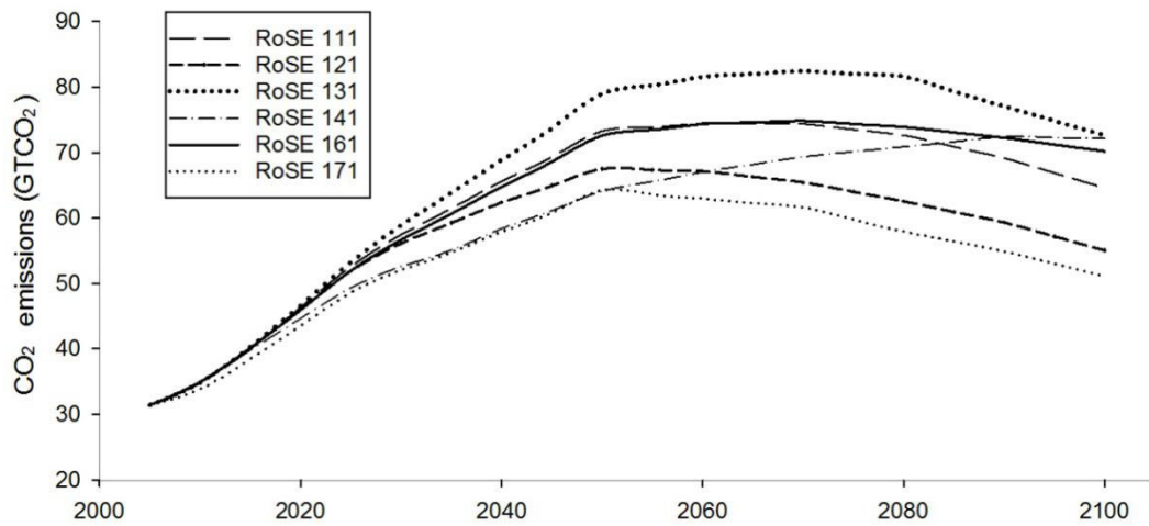
Fig. 4 CO 2 emissions in six global BAU scenarios
