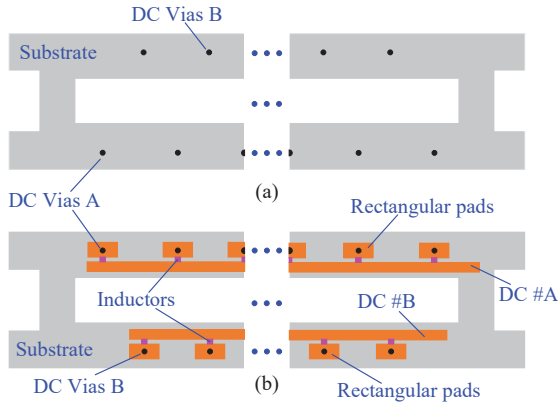
Fig. 2. The lower substrate of the fixed-frequency beam scanning CRLH LWA. (a) Top layer of the lower substrate. (b) Biasing layer.
