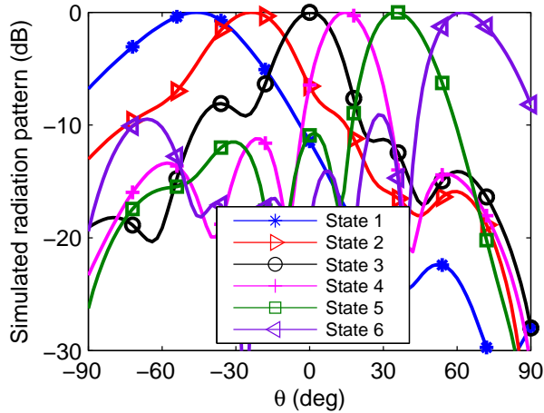
Fig. 4. Simulated radiation patterns for antenna's six operating states at 5 GHz.
