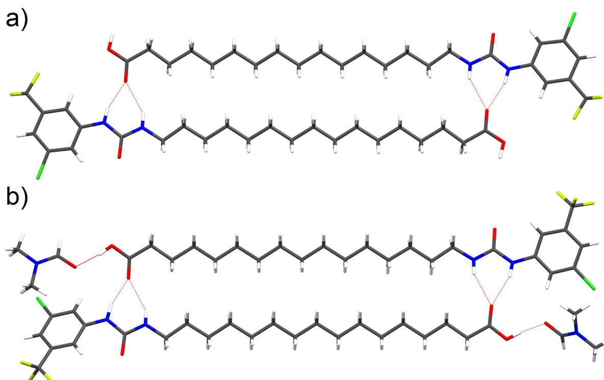
Figure 6. Single crystal structure of 6 (a, CCDC 1998411) and 6-DMF solvate (b, CCDC 1998415) with hydrogen bonds represented by red dashed lines.
