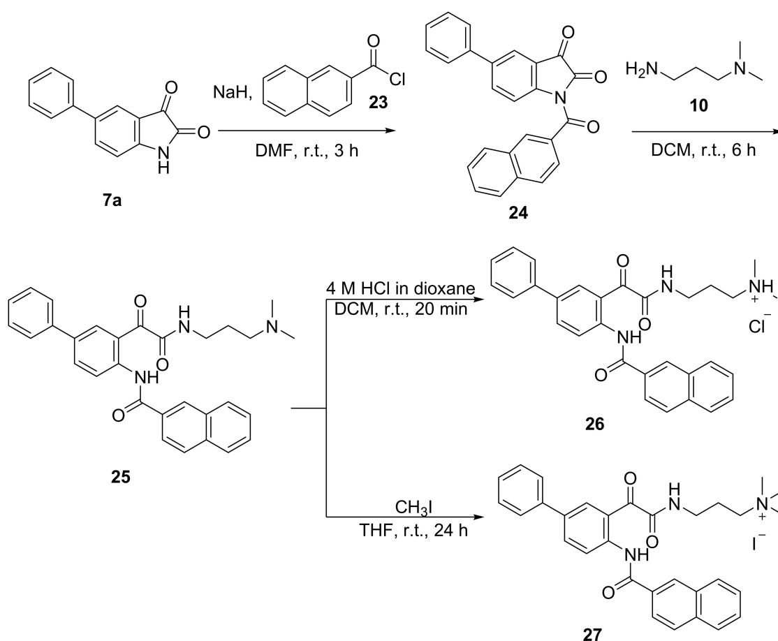
Scheme 4. Synthesis of N -naphthoyl glyoxamide derivative 25 and its corresponding tertiary ammonium chloride salt 26 and quaternary ammonium iodide salt 27 .
