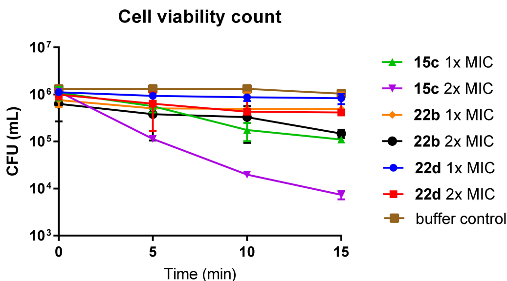
Figure 6. Cell viability count of S. aureus in the presence of compound 15c, 22b and 22d at 1x and 2x their MIC.
