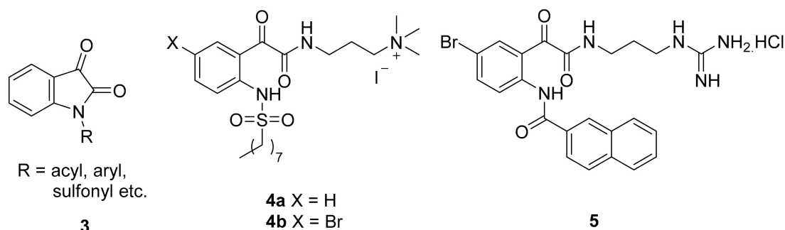
Figure 2. Structures of N -substituted isatin 3 and phenylglyoxamide derivatives 4–5 .
