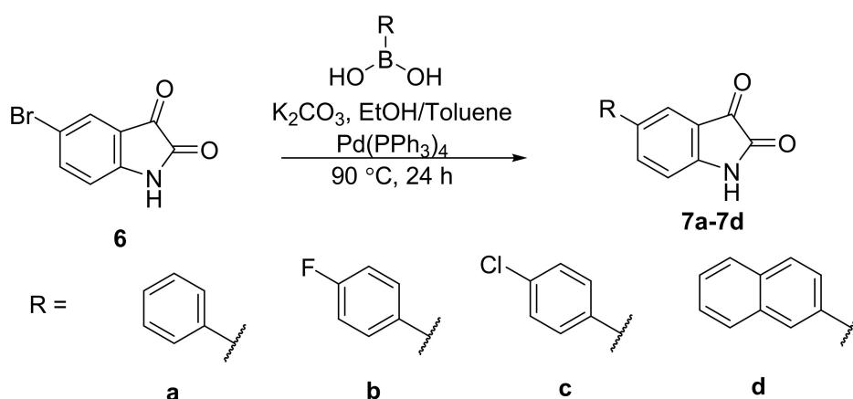
Scheme 1. Synthesis of 5-arylisatins 7a–7d .
