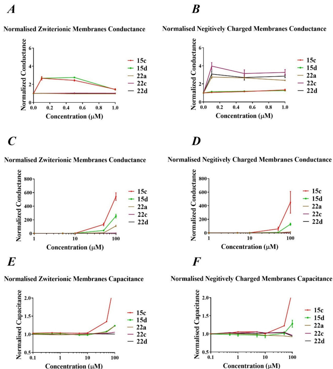
Figure 7. (A) Changes in membrane conductance caused by the addition of the compounds at concentrations less than 1 \mu\text{M} in (A) zwitterionic POPC tBLMs, and (B) tBLMs containing 30% negatively charged POPG lipids. Large increases in membrane conduction due to select compounds are also visible at higher concentrations (1–100 \mu\text{M} ) in (C) zwitterionic POPC tBLMs, and (D) tBLMs containing 30% negatively charged POPG lipids. Large increases in membrane capacitance in (E) zwitterionic tBLMs, and (F) negatively charged tBLMs, suggests that high concentrations of compounds lead to massive disruption of the lipid bilayers. Error bars represent the standard errors from n = 3 replicates for each compound, with the exception of 15c, which is n = 2 .
