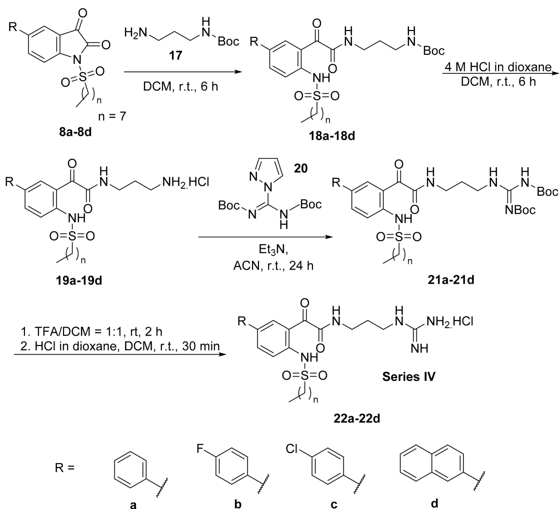
Scheme 3. General synthetic scheme for the synthesis of series IV guanidinium hydrochloride salts 22 .
