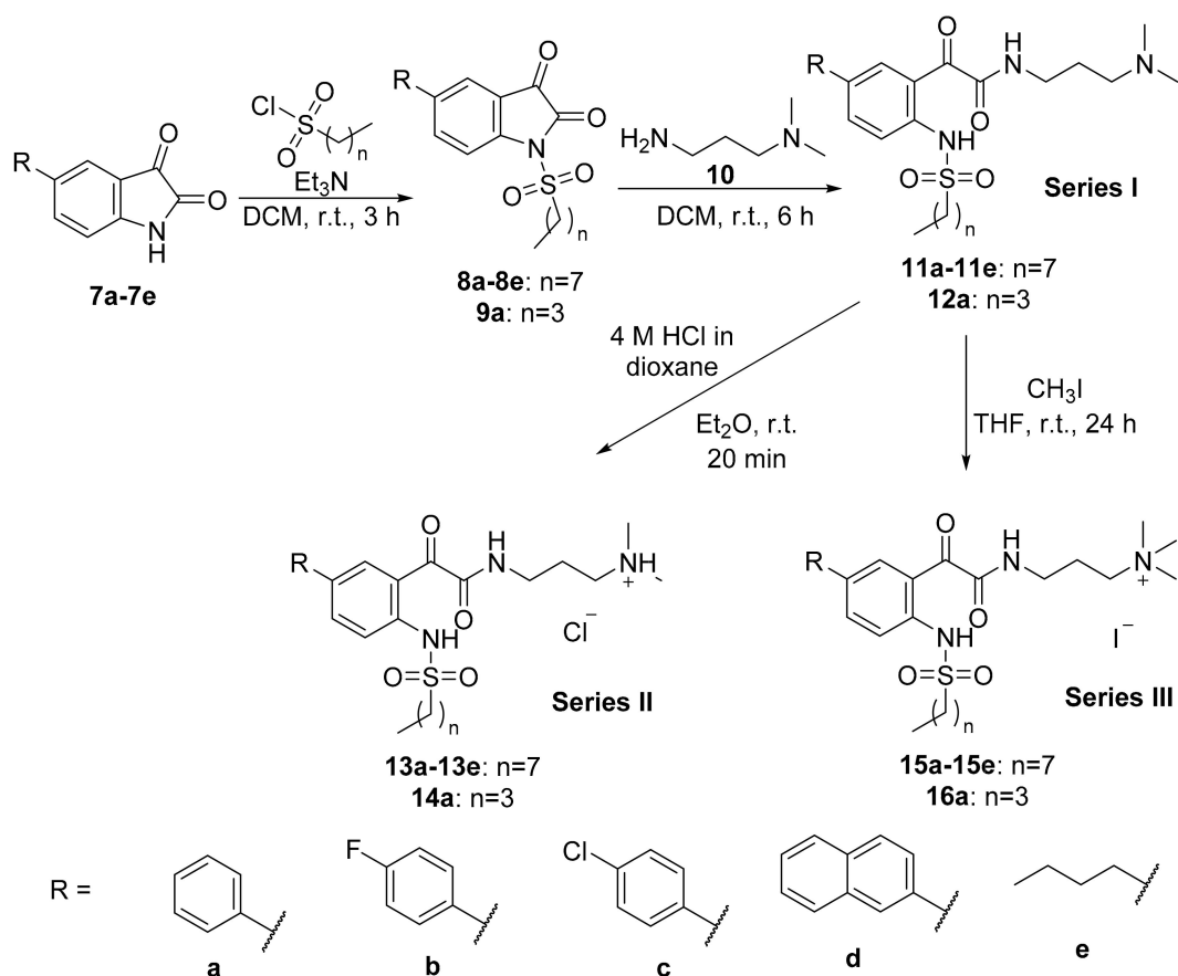
Scheme 2. General synthetic scheme for the synthesis of series I glyoxamide derivatives 11–12 , series II tertiary ammonium chloride salts 13–14 and series III quaternary ammonium iodide salts 15–16 .
