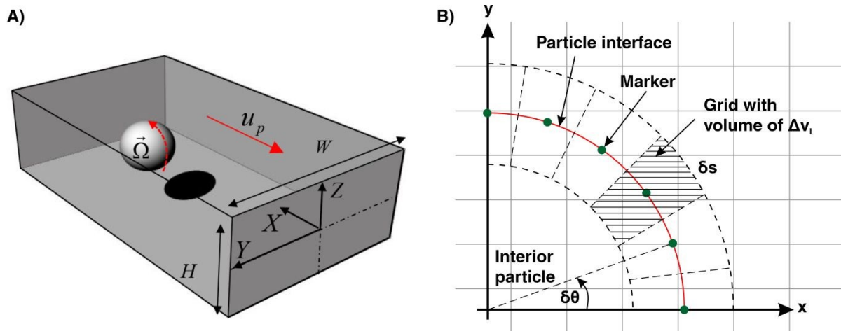
Fig. 3 A) Schematic illustration of particle motion in a part of the channel. The surface of particle rotates with an angular velocity of \Omega , and walls have the backward velocity of u_p . Reprinted from [50] with the permission of AIP Publishing. B) Representation of the Eulerian and distribution of Lagrangian grids. Eulerian grid is shown with fix staggered Cartesian grid with gray color. Lagrangian grid is represented by a set of green markers, which are distributed evenly over the surface of the particle with an element size of \Delta v_l .
