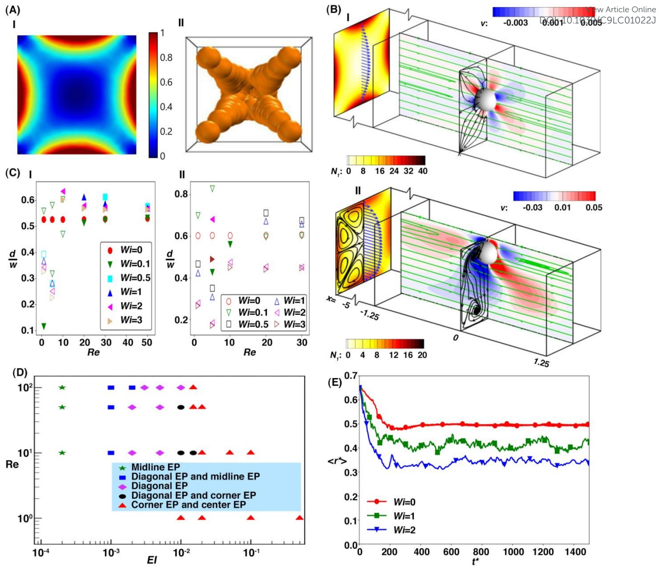
Fig. 9 A) Migration of particles in a straight channel with the viscoelastic fluid flow. I. Distribution of the shear rate in the cross-section of the channel. II. Particles move toward the minimum shear rate region. Reprinted from [88], with the permission of AIP Publishing. B) Investigation of fluid behavior and particle equilibrium position in I. Oldroyd-B II. and Giesekus fluids [92]. C) the distance of the off-center lateral position of particles from the center of the channel along the I. main axis and II. diagonal of the channel for all ranges of Wi and Re . Stable equilibrium positions are identified by filled symbols, whereas unstable ones are represented by unfilled symbols [89]. D) focusing pattern of a particle with a blockage ratio of 0.15 under different conditions of EI and Re [90]. E) Increasing in Wi leads to relocation of the cells toward the centerline [93].
