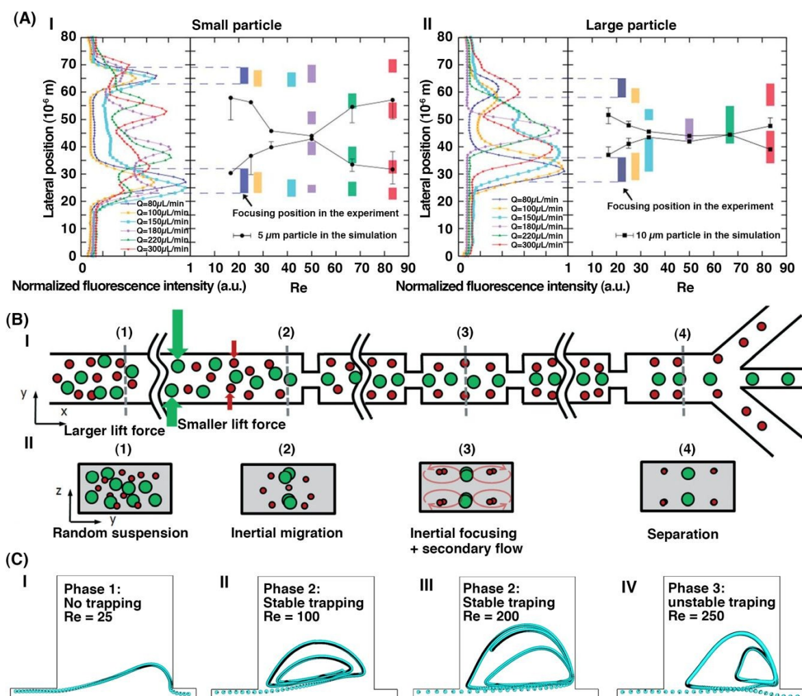
Fig. 13 A) The comparison of the lateral position of particles with different sizes in a channel. Data shown in the figure is obtained experimentally and numerically. Reproduced from Ref. [126] with permission from The Royal Society of Chemistry. B) I. Schematic illustration and the design principle of the proposed contraction expansion microchannel by Wu and co-workers. II. randomly dispersed particles were first focused due to the inertial effect. Next, at the presence of contraction-expansion arrays, secondary flows were induced resulted in the migration of small particles to the side of channel walls while maintaining large particles near the centerline of the channel. Afterward, each stream was collected from separate outlets. Reproduced from Ref. [130] with permission from The Royal Society of Chemistry. C) Three particle entrapping phases I. no trapping, II. stable trapping, and III. Unstable trapping.
