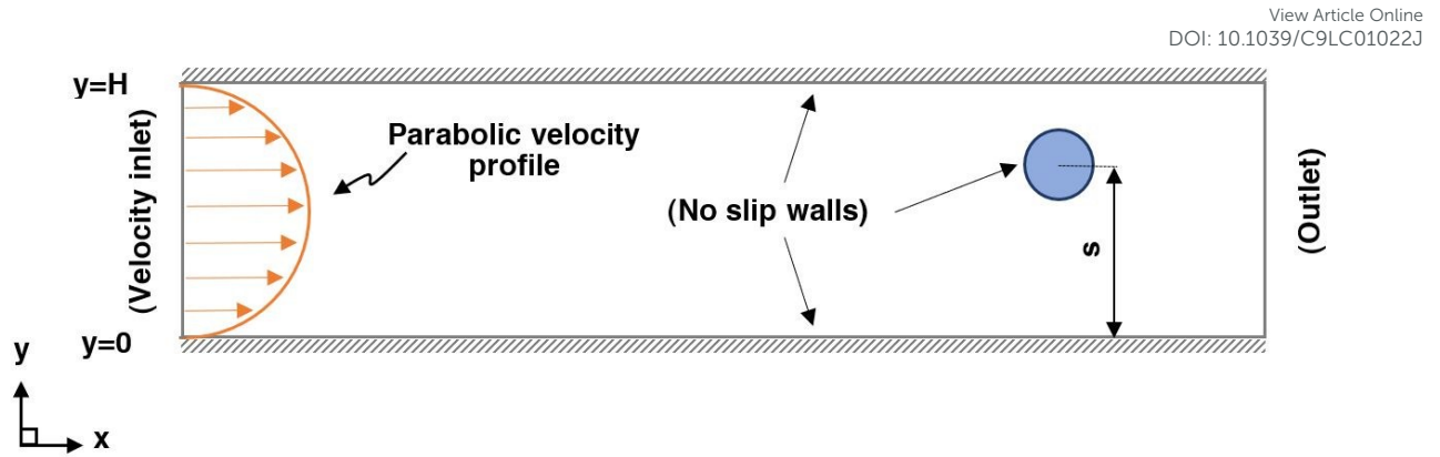
Fig. 2 The schematic view of a cylindrical particle inside the confine channel flow
