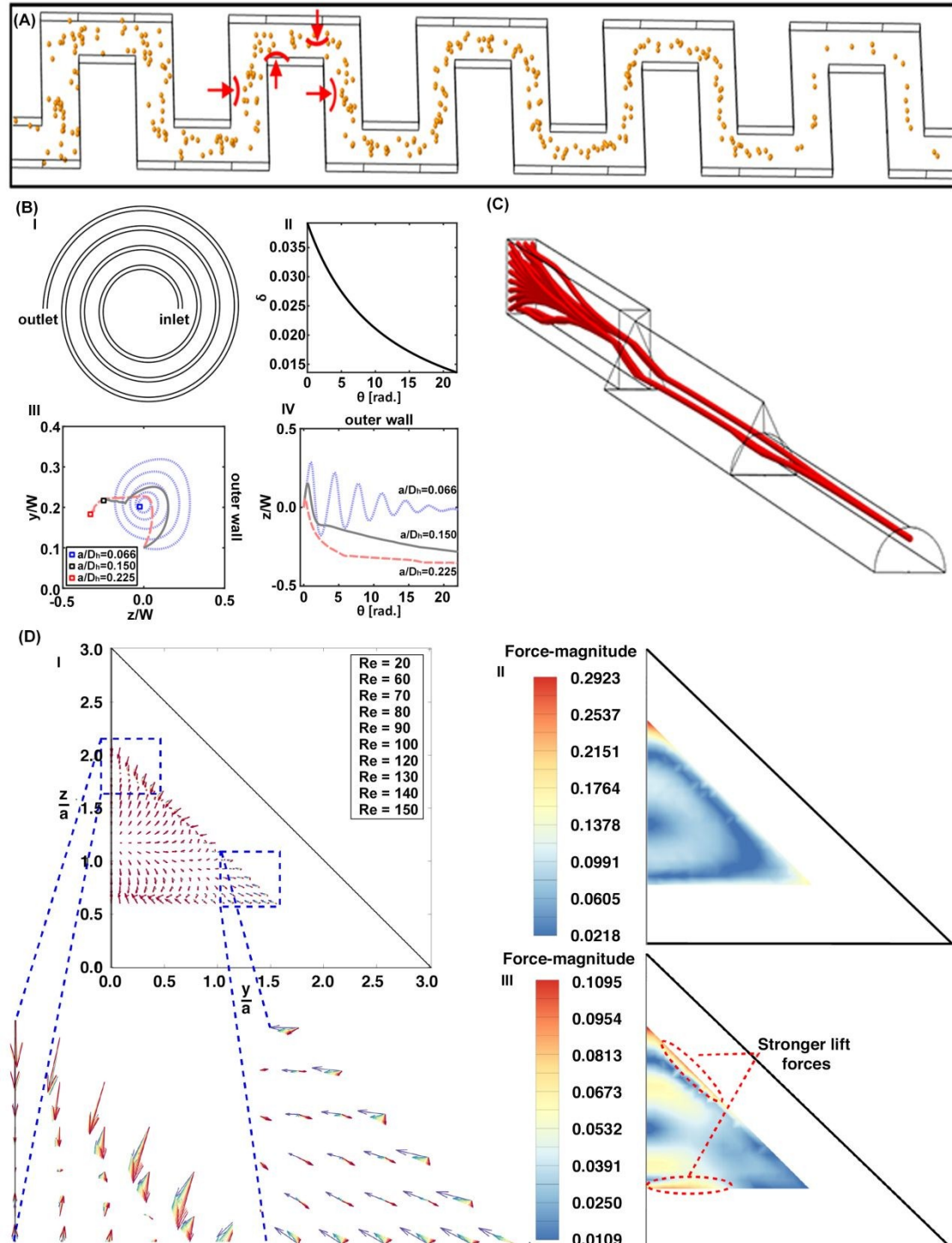
Fig. 8 Inertial microfluidics in non-straight channels. A) Particle focusing in the serpentine channel; red arrows show the direction of drag forces inside the channel. Reprinted from [50] with the permission of AIP Publishing. B) I. Illustration of a spiral II. variation of the channel curvature ( \delta ) along the length of channel (in polar coordinates). III. The cross sectional particle trajectory for three different particles.
