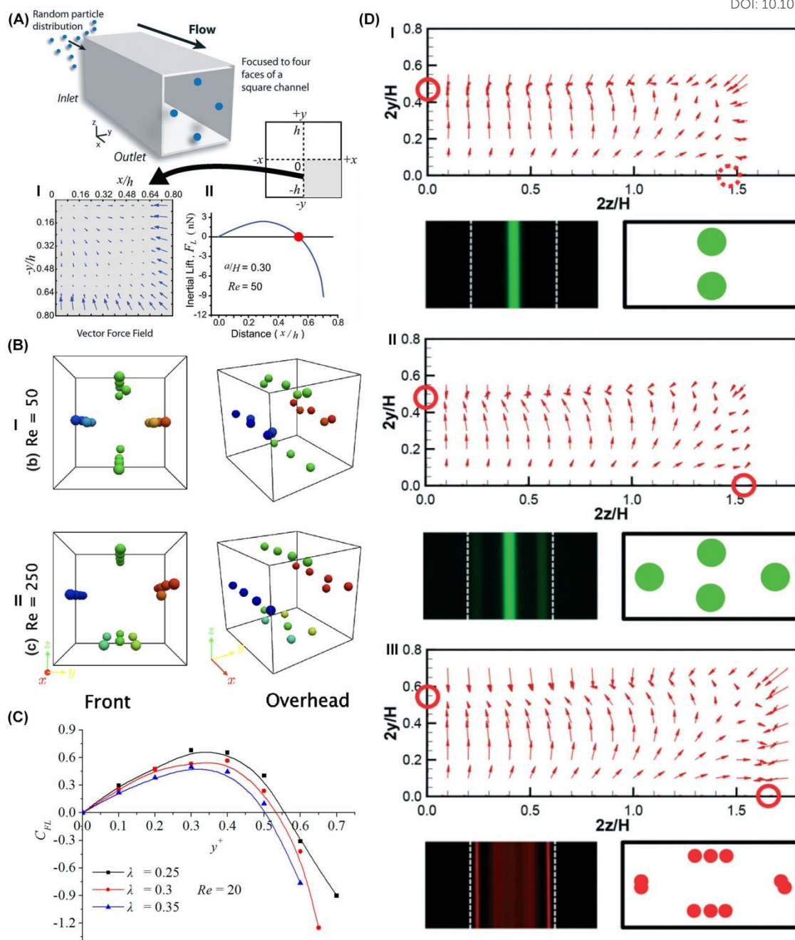
Fig. 5 Inertial microfluidics in the straight channels with a rectangular and square cross-sections. A) The lift force acting on the particle in a square channel. Reproduced from Ref. [10] with permission from The Royal Society of Chemistry. I) distribution of the lift force in a quarter of the cross-section. II) Value of inertial lift force from the center to the wall. https://doi.org/10.1103/PhysRevLett.102.094503 . B) The focusing pattern of particles in a channel with a square cross-section at low (I) and high (II) Re [56]. C) By increasing the particle size (blockage ratio), the equilibrium position of particle moves toward the center [57]. D) Distributions of lift force acting on the particle in a rectangular channel with an aspect ratio of two under various Re and particle sizes. Reproduced from Ref. [38] with permission from The Royal Society of Chemistry. I) Only the centers of the long walls are stable equilibrium positions (the blockage ratio (a/H) = 0.3 and Re=100 ). II) Stable equilibrium particle position at Re=200 and blockage ratio of 0.3 III) By increasing Re to
