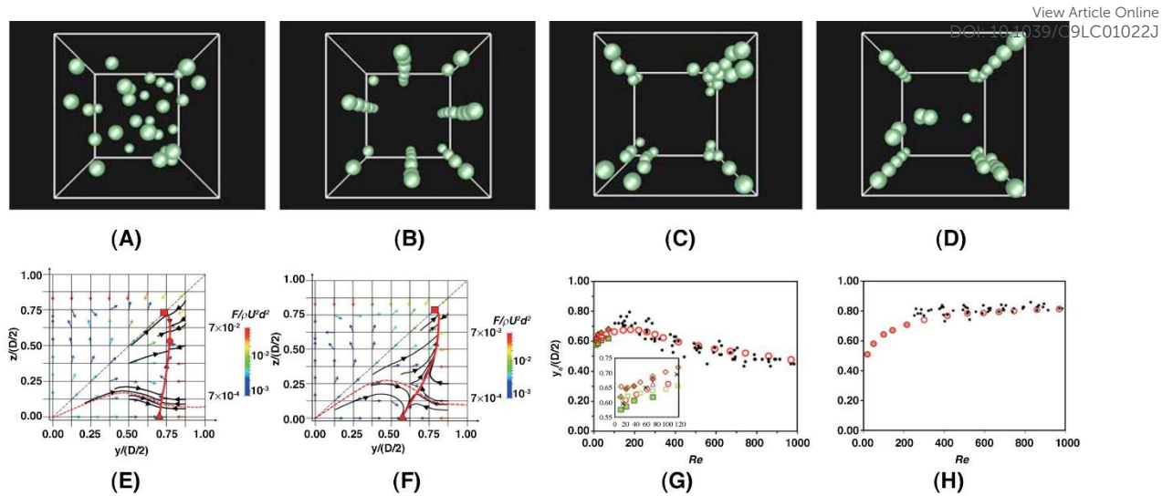
Fig. 10 A) Initial distribution of particles leads to different equilibrium positions based on Re . Particle equilibrium positions for Re of B) 100, C) 500, and D) 1000. Based on results presented by Chun and Ladd [104], at Re = 100 , particles migrated to the eight equilibrium positions. For Re = 500 , particles migrated to one of four stable locations near the corner of square duct, while for Re = 1000 , the particle equilibrium configuration changed. Reprinted from [104], with the permission of AIP Publishing. Map of lateral forces for Re of E) 260 and F) 514 calculated by Nakagawa and co-workers [105] who showed that the particle behavior and equilibrium positions change by increasing Re . Equilibrium position in G) channel face and H) channel corner. Circles are the results of their study, while experimental results are indicated by other shapes.
