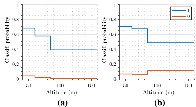
Fig. 13 Sensor models for our trained classifier for the a ‘Lake’ and b ‘BRV’ classes. The blue and orange curves depict the probability of observing class label ‘1’, given that the map contains ‘1’ or ‘0’, i.e., true and false positives, respectively. Note that the false positive probability can decrease with altitude as the classifier becomes more conservative with true outputs (Color figure online)
