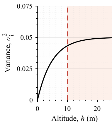
Fig. 3 Inverse sensor noise model for a camera providing measurements as \mathcal{N}(\mu_{s,i}, \sigma_{s,i}^2) with a = 0.2, b = 0.05 in Eq. (7). The uncertainty \sigma_{s,i}^2 increases with h to represent degrading image quality. The dotted line at h = 10 m indicates the altitude above which image resolution scales down by a factor of 2
