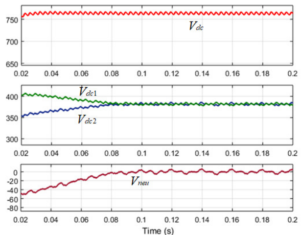
Fig. 7: Midpoint voltage control waveform with different capacitors value
