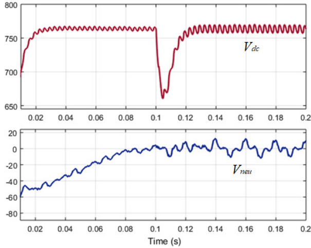
Fig. 8: DC side voltage and neutral point voltage during load change
