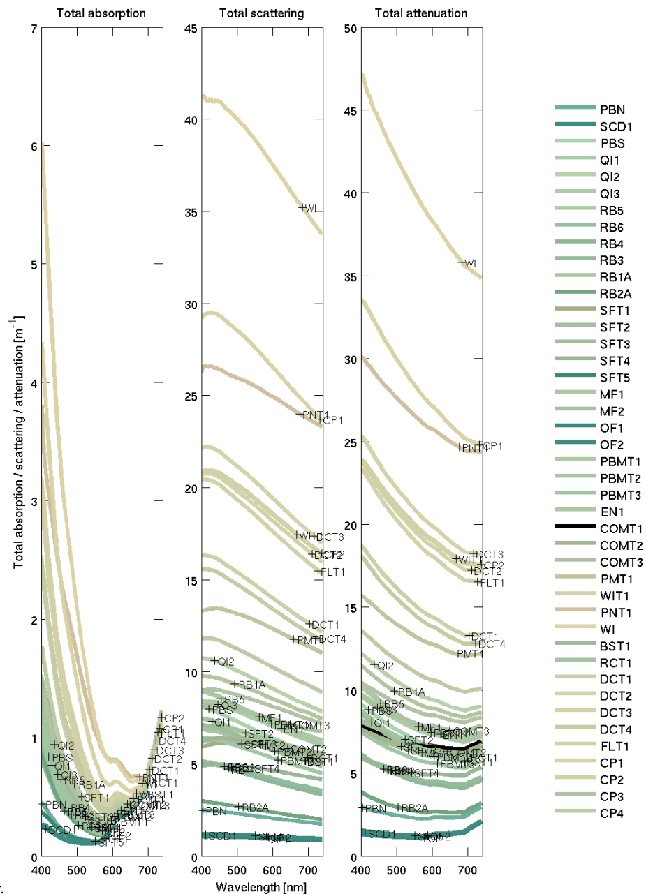
IOPs from Gladstone Harbour.
