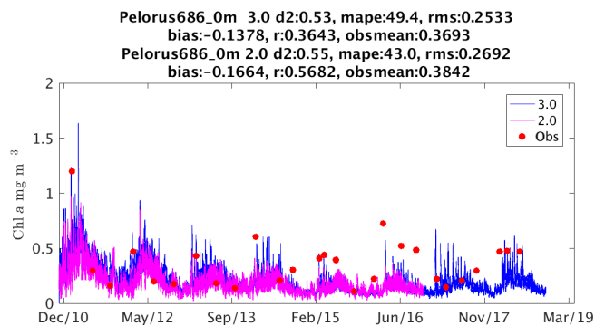
Figure 14. Observed surface chlorophyll concentration from chlorophyll extraction (red dots) at the Pelorus Island Marine Monitoring Program site ( 18^{\circ}33' \text{ S} , 146^{\circ}29' \text{ E} ) with a comparison to configurations vB2p0 (pink line) and vB3p0 (blue line). Statistics listed include the Willmott d2 metric (Willmott et al., 1985), mean absolute percent error (MAPE) and RMSE.
