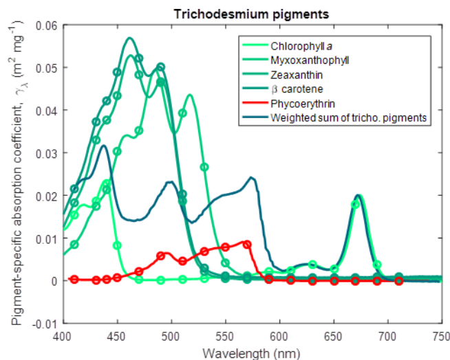
Figure 7. Pigment-specific absorption coefficients for the dominant pigments found in Trichodesmium determined using laboratory standards in solvent in a 1 cm vial. The aqua line represents the weighted sum of the photosynthetic pigments (Eq. 5), with the weighting calculated from the ratio of each pigment concentration to chlorophyll a . See Fig. 5 for more details. Myxoxanthophyll was dissolved in acetone.
