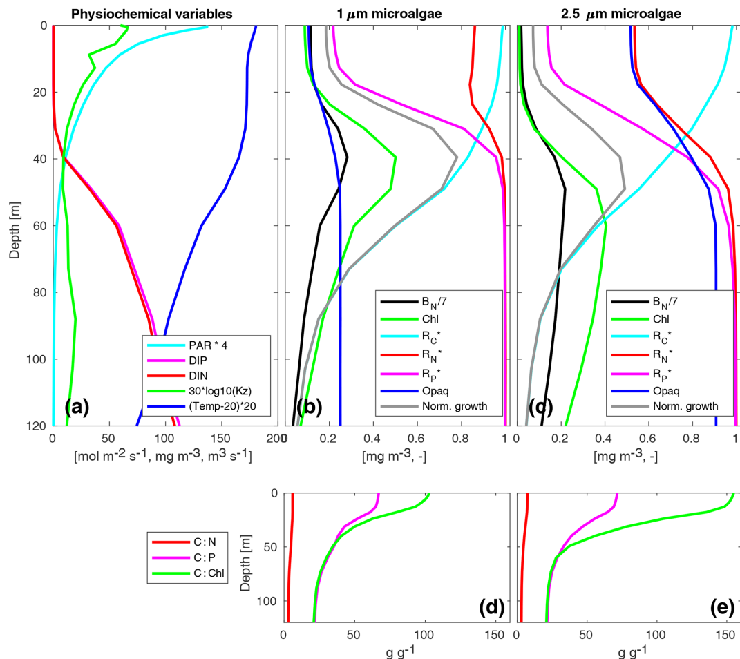
Figure 13. Vertical profiles of physiochemical variables (a) and physiological variables from 1 μm (b, d) and 2.5 μm (c, e) radii microalgae. Panel (a) shows photosynthetically available radiation (PAR; mol\ m^{-2}\ s^{-1} ), dissolved inorganic phosphorus (DIP; mg\ P\ m^{-3} ), dissolved inorganic nitrogen (DIN; mg\ N\ m^{-3} ), vertical diffusivity ( K_z ; m^3\ s^{-1} ) and temperature ( ^{\circ}C ). Panels (b) (1 μm) and (c) (2.5 μm) show biomass of structural material in nitrogen ( B_N ; mg\ N\ m^{-3} ), chlorophyll a concentration (Chl; mg\ Chl\ a\ m^{-3} ), normalised reserves of fixed carbon ( R_C^* ), nitrogen ( R_N^* ) and phosphorus ( R_P^* ), cell opaqueness (absorption cross-section divided by projected area, \alpha/(\pi r^2) ) and normalised growth rate of R_C^* R_N^* R_P^* . Panels (d) (1 μm) and (e) (2.5 μm) show stoichiometric ratios of carbon to nitrogen (C : N), phosphorus (C : P) and chlorophyll (C : Chl a ). PAR, K_z , temperature and B_N are all scaled for plotting.
