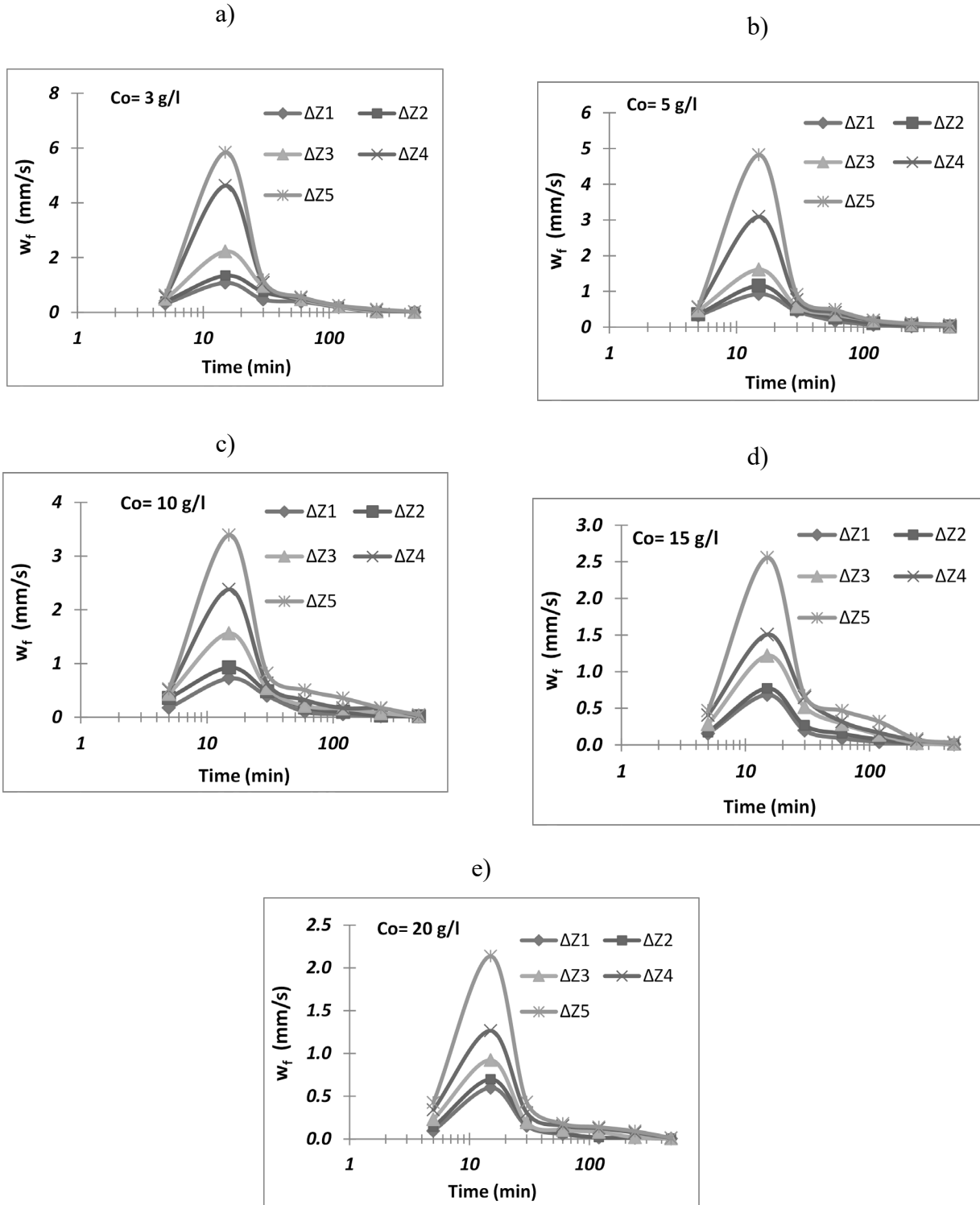
Fig. 6. Sediment settling velocity Changes versus time (a: C_o = 3 g/l , b: C_o = 5 g/l , c: C_o = 10 g/l , d: C_o = 15 g/l , e: C_o = 20 g/l)
