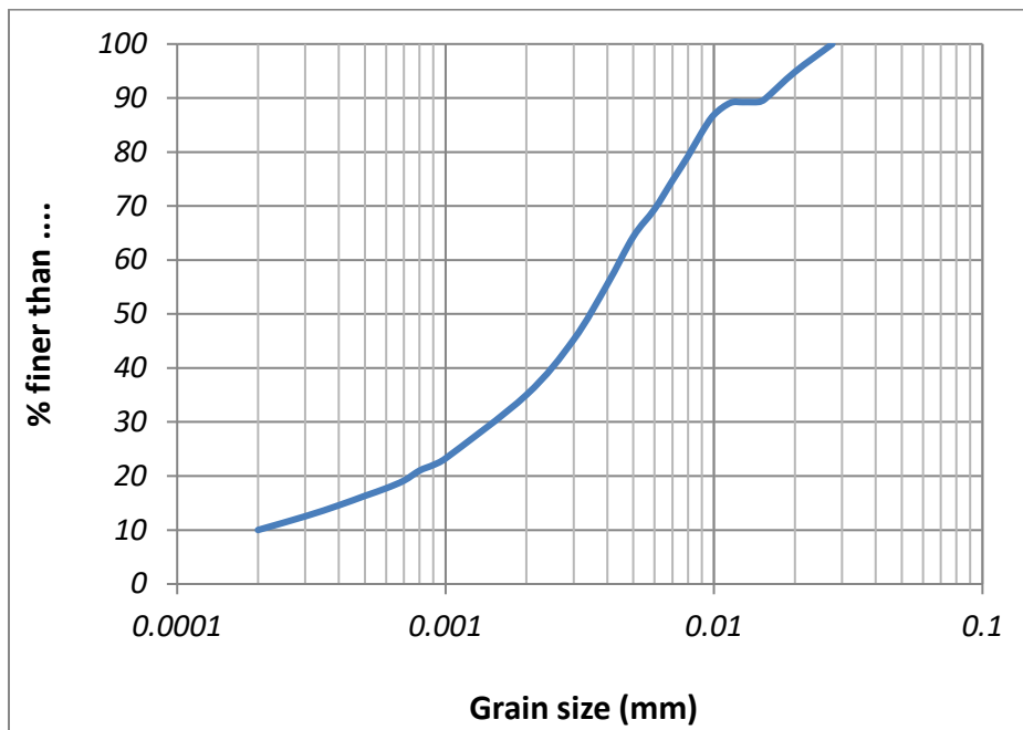
Fig. 2. The grain size distribution curve for sediment used in the experiments.
