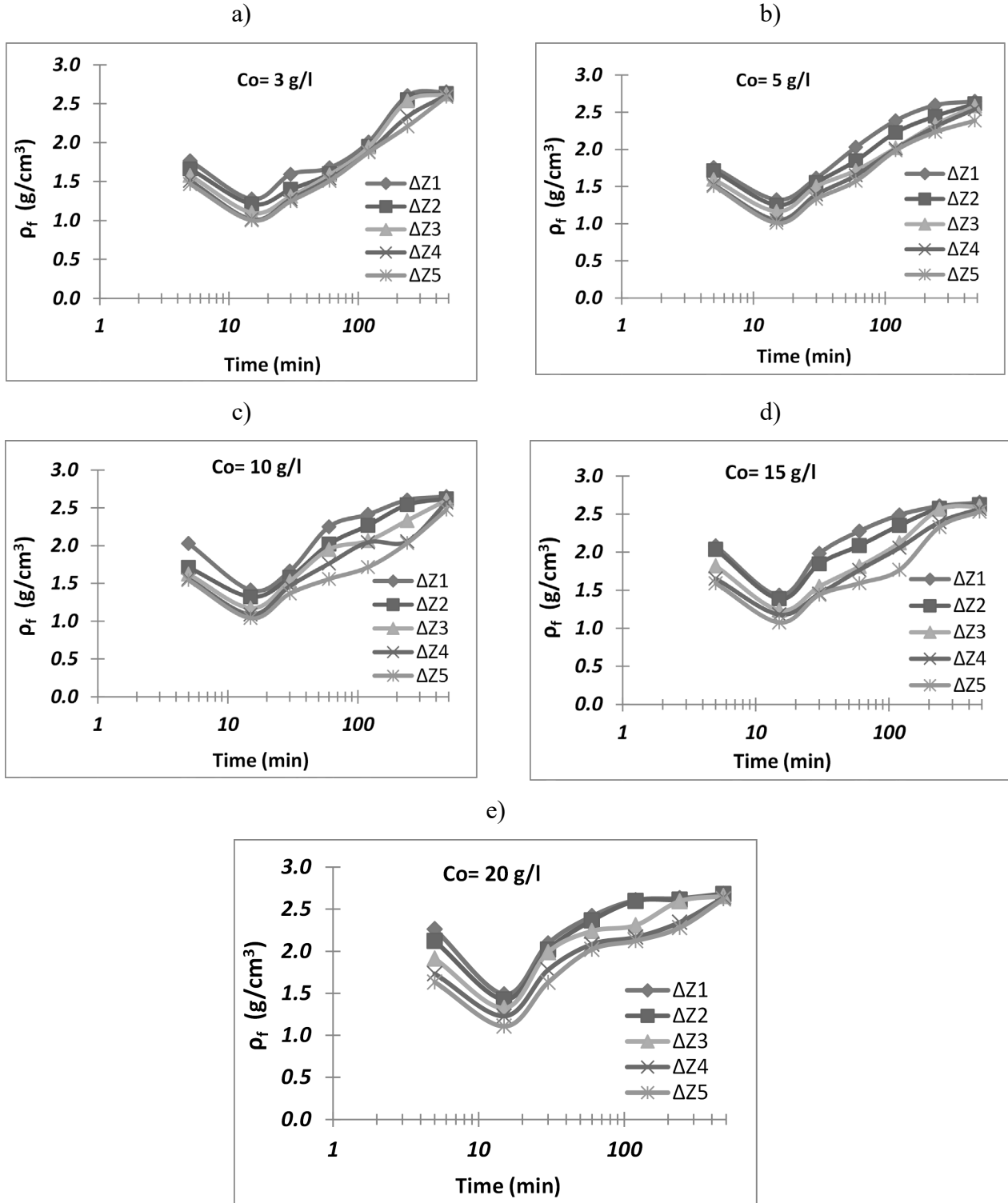
Fig. 7. Time Variation of the flocc wet bulk density (a: C_o = 3 g/l , b: C_o = 5 g/l , c: C_o = 10 g/l , d: C_o = 15 g/l , e: C_o = 20 g/l)
