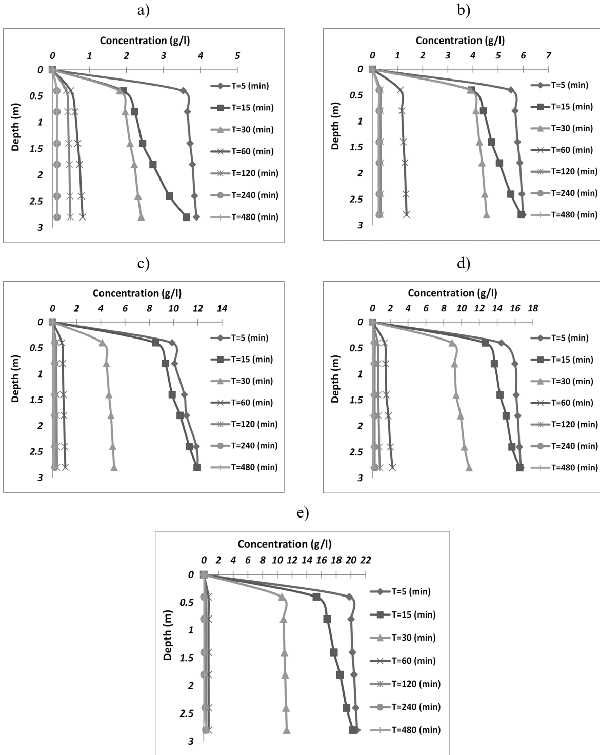
Fig. 3. Concentration depth distribution for the conducted experiments
