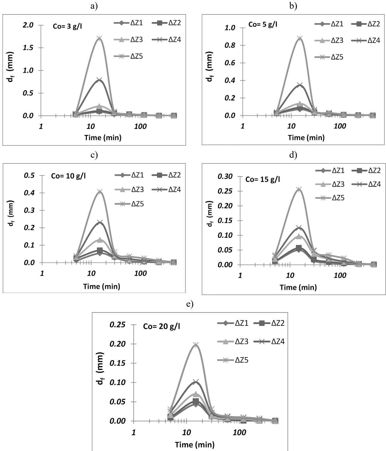
Fig.8. Time Variation of the floc diameter (a: C_o= 3 g/l , b: C_o= 5 g/l , c: C_o= 10 g/l , d: C_o= 15 g/l , e: C_o= 20 g/l)
