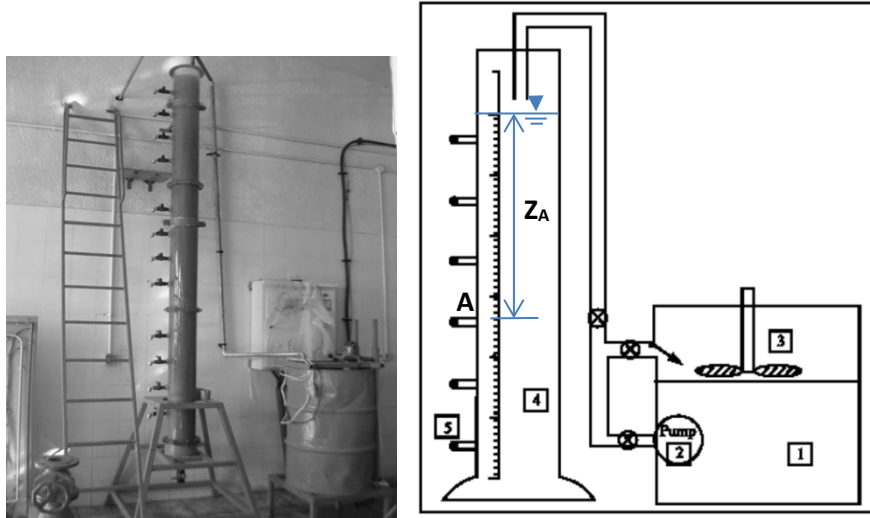
Fig. 1. Settling column, (1) storage tank ( 0.4 \text{ m}^3 ) for mixing water and sediment with desirable density, (2) pump to deliver water to settling column, (3) a mixer connected to appropriate electric motor, (4) plexy glass settling cylinder, 3 m height and 0.3 m diameter, and (5) sampling outlets, 0.3 m apart
