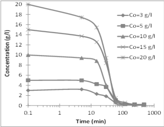
Fig.4. Changes with time in sediment concentration in the conducted experiments
