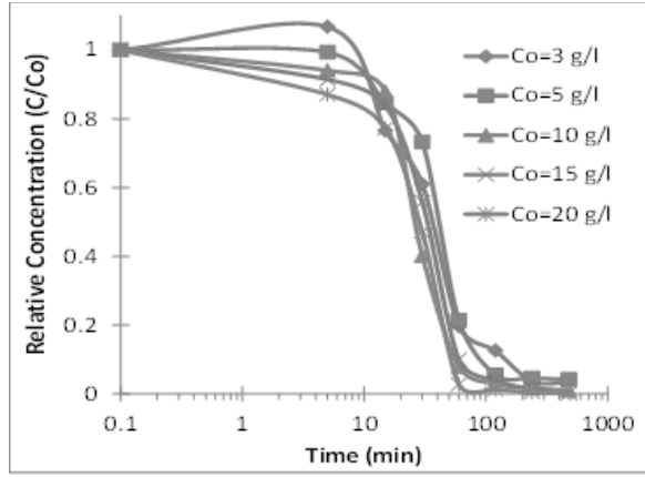
Fig. 5. Changes with time in dimensionless sediment concentration in the conducted experiments
