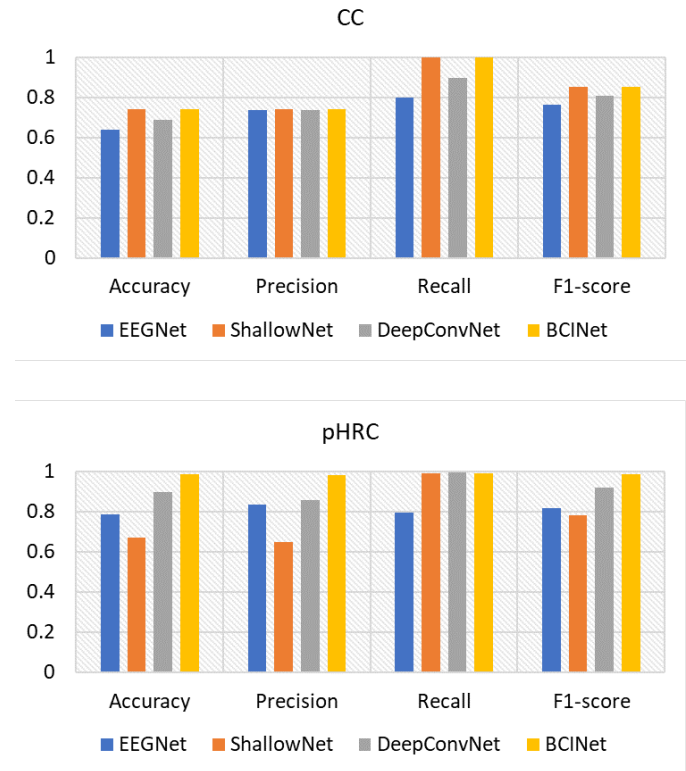
Fig. 5. Accuracy, precision, recall, and F1-score for EEGNet, ShallowNet, DeepConvNet, and BCINet on CC and pHRC-dataset
