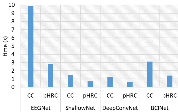
Fig. 4. Time required for prediction in EEGNet, ShallowNet, DeepConvNet, and BCINet on CC and pHRC-dataset
