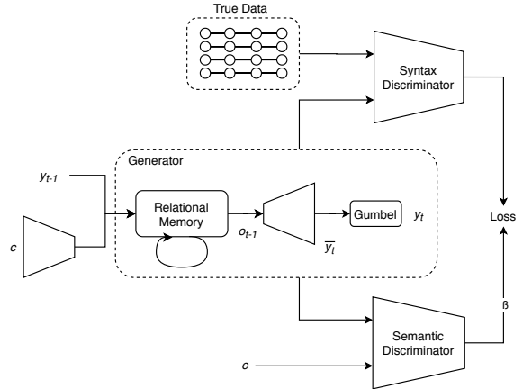
Figure 1: CTERM-GAN architecture
