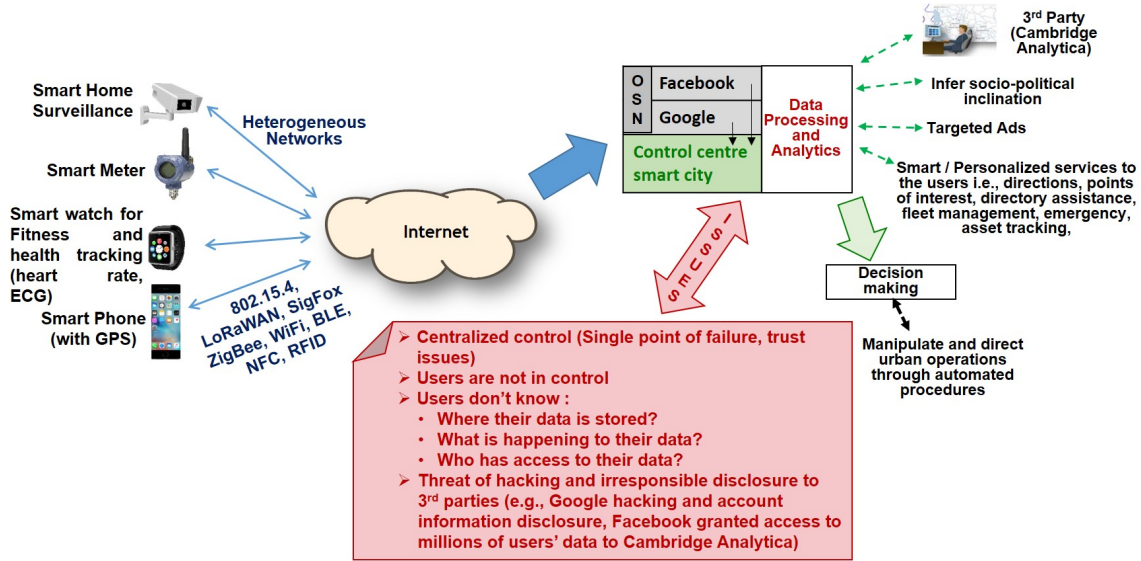
Figure 1: Issues in the smart city environment
