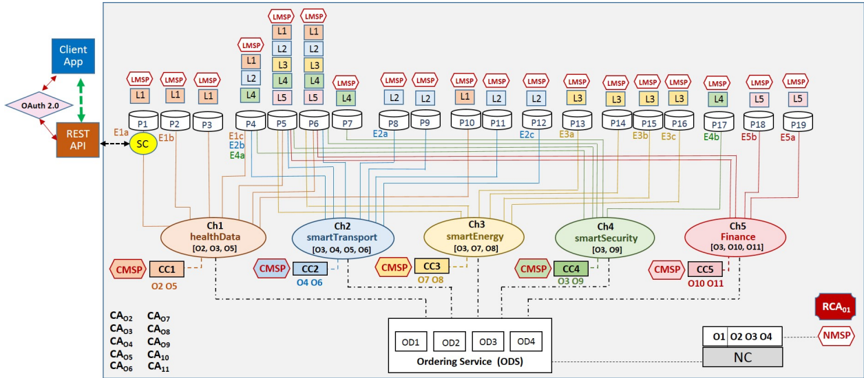
Figure 3: Smart city blockchain-network architecture
