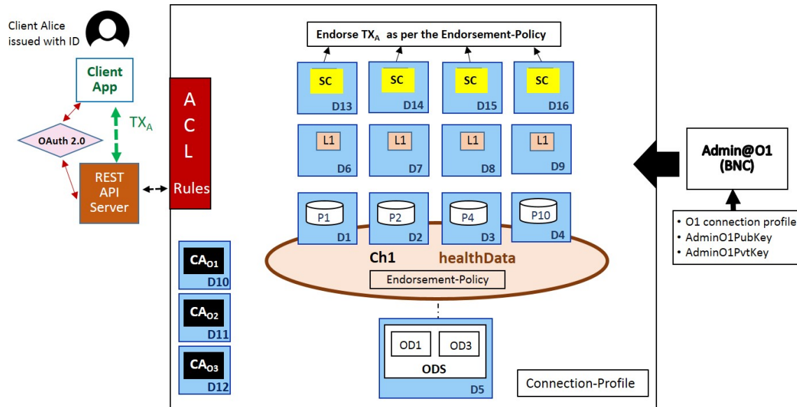
Figure 8: Elements of PrivySharing network security
