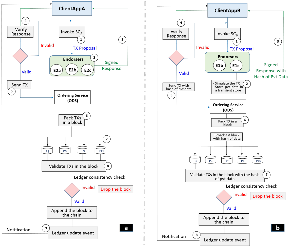
Figure 5: a) Plain TX flow, and b) Private data TX flow
