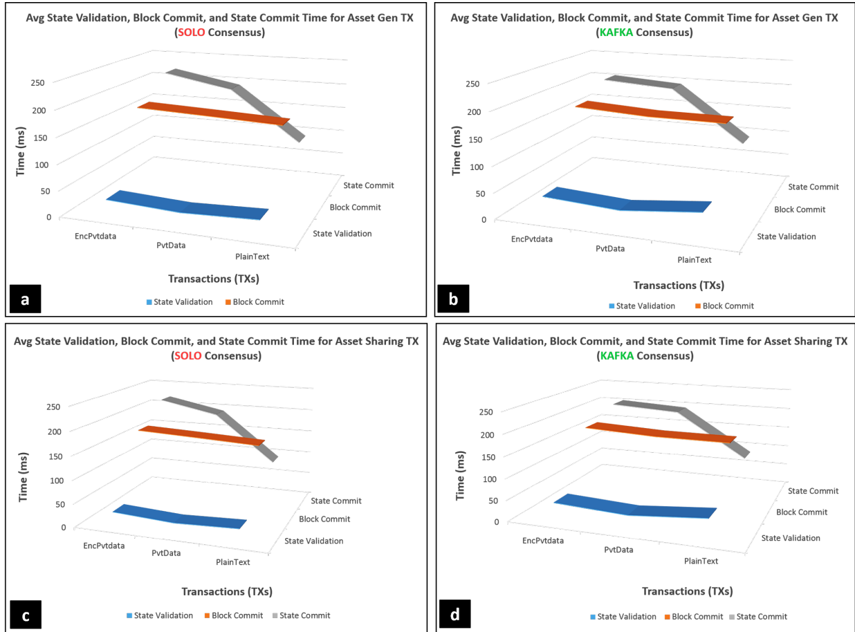
Figure 18: Comparison of State validation, Block commit, and State commit avg time
