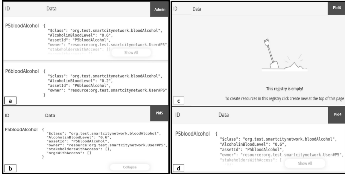
Figure 14: Validation of assets access control
