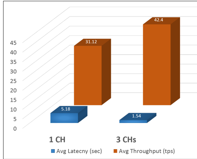
Figure 19: Comparison of Avg Latency and Avg Throughput in One-Ch and Three-Ch Scenario
