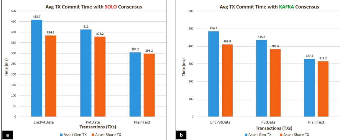
Figure 17: Avg TX Commit Time
