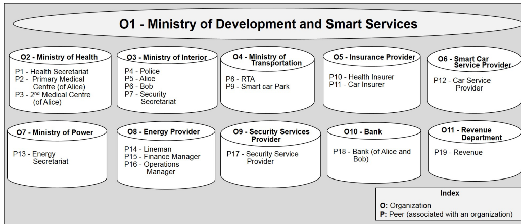
Figure 2: Network participants
