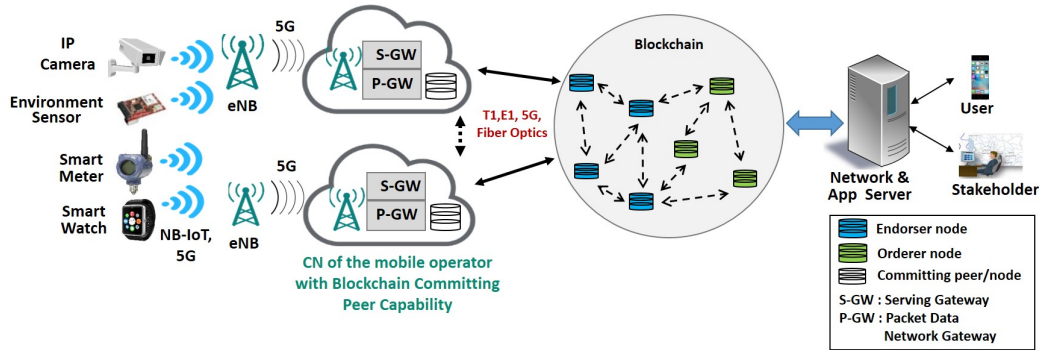
Figure 22: Integration of Blockchain with MEC
