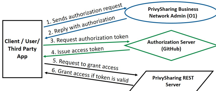
Figure 10: PrivySharing REST server OAuth protocol
