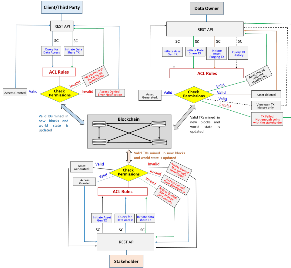
Figure 4: Smart Contract TXs
