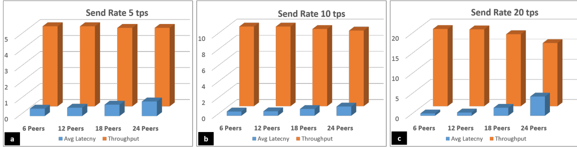
Figure 21: Correlation between number of peers and network throughput at the send rate of (a) 5 tps, (b) 10 tps, and (c) 20 tps
