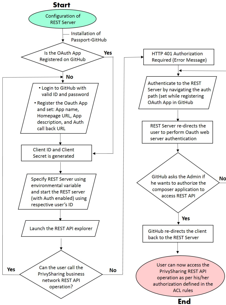
Figure 11: PrivySharing REST server OAuth flowchart
