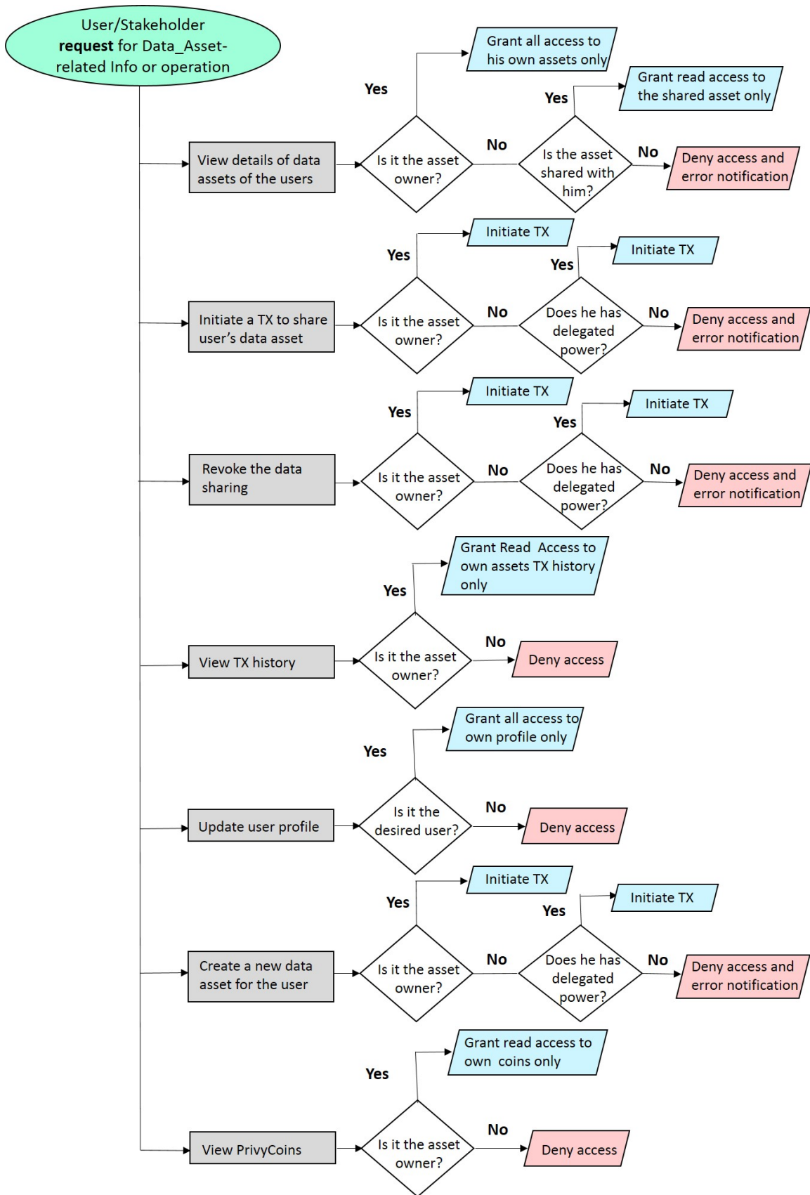
Figure 9: ACL rules
