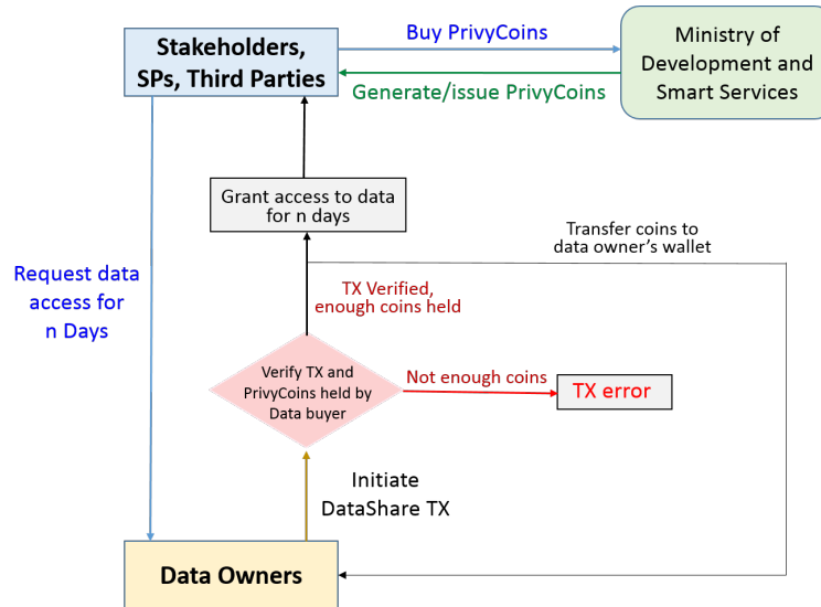
Figure 6: Reward mechanism based on PrivyCoins
