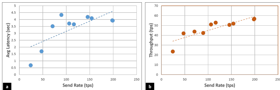
Figure 20: a) Correlation between TX send rate and latency. b) Relation between TX send rate and network throughput
