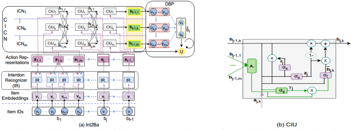
Figure 1: (a) The Int2Ba model mainly consists of three components: Intention Recognizer (IR), CICN and DBP (the circle with arrow means the basket generation is iterative); (b) each CIU in CICN introduces an attention model (denoted as A ) and an influence gate ( \sigma_s in green color) to attentively integrate the other intention states and then selectively absorb them into the current intention transition respectively.
