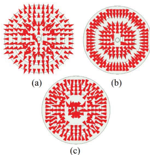
Fig. 3. Simulated current distribution on the proposed patch surface at; (a) 3.5 GHz ( TM_{01} ); (b) 6 GHz ( TM_{02} ) and; (c) 7 GHz ( TM_{03} ).
