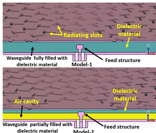
Fig. 1: Cross-section view of the two CP-RLSA antennas with two different waveguide configurations.
