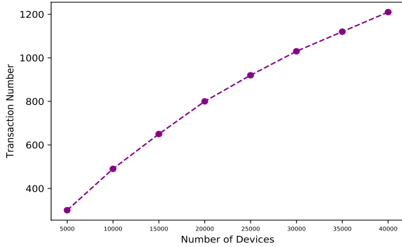
Fig. 5. Transaction Number with respect to Number of devices
