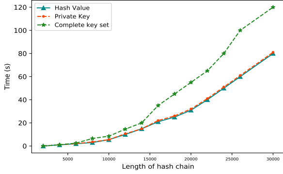
Fig. 4. Time required for Key pair generation
