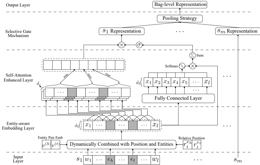
Figure 1: The framework of our approach (i.e. SeG) that consisting of three components: 1) entity-aware embedding 2) self-attention enhanced neural network and 3) a selective gate. Note, tokens e_h and e_t with gray background mean the head entity and tail entity of this sentence.
