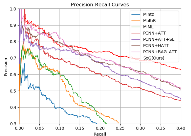
Figure 2: Performance comparison for proposed model and previous baselines in terms of precision-recall curves
