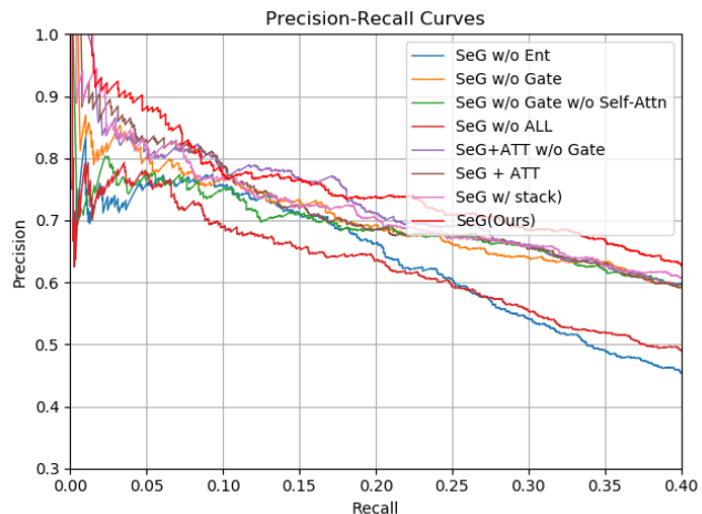
Figure 3: Performance comparison for ablation study under precision-recall curves
